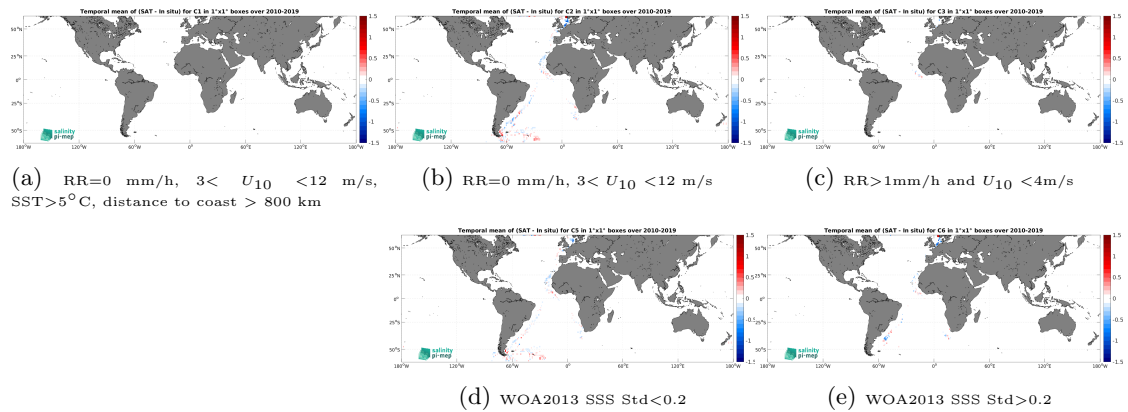
Figure 12: Temporal mean gridded over spatial boxes of size 1^\circ \times 1^\circ of \Delta\text{SSS} (CCI SSS L4 Merged-OI v3.2 - 7-day running (ESA) - TSG (Polarstern)) for 5 different subdatasets corresponding to:RR=0 mm/h, 3 < U_{10} < 12 m/s, SST >5^\circ\text{C} , distance to coast > 800 km (a), RR=0 mm/h, 3 < U_{10} < 12 m/s (b), RR >1 mm/h and U_{10} < 4 m/s (c), WOA2013 SSS Std <0.2 (d), WOA2013 SSS Std >0.2 (e).
