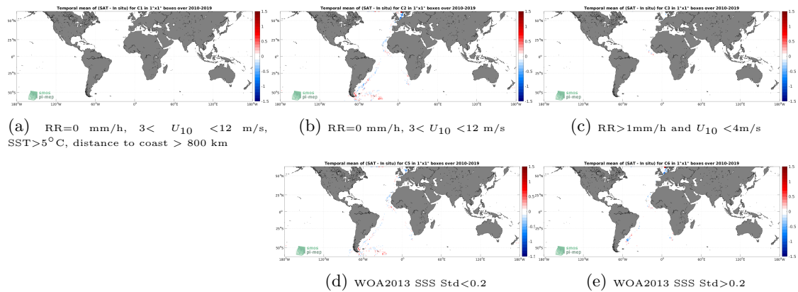
Figure 12: Temporal mean gridded over spatial boxes of size 1^\circ \times 1^\circ of \Delta SSS (CCI SSS L4 Merged-OI v3.2 - 7-day running (ESA) - TSG (Polarstern)) for 5 different subdatasets corresponding to:RR=0 mm/h, 3 < U_{10} < 12 m/s, SST >5^\circ\text{C} , distance to coast > 800 km (a), RR=0 mm/h, 3 < U_{10} < 12 m/s (b), RR >1 mm/h and U_{10} < 4 m/s (c), WOA2013 SSS Std <0.2 (d), WOA2013 SSS Std >0.2 (e).
