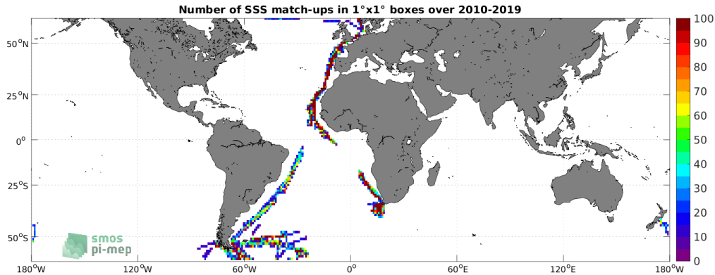
Figure 4: Number of SSS match-ups between TSG (Polarstern) SSS and the CCI SSS L4 Merged-OI v3.2 - 7-day running (ESA) SSS product for the SMOS coastal zone (<800km) 60N-60S Pi-MEP region over 1^\circ \times 1^\circ boxes and for the full satellite product period.
