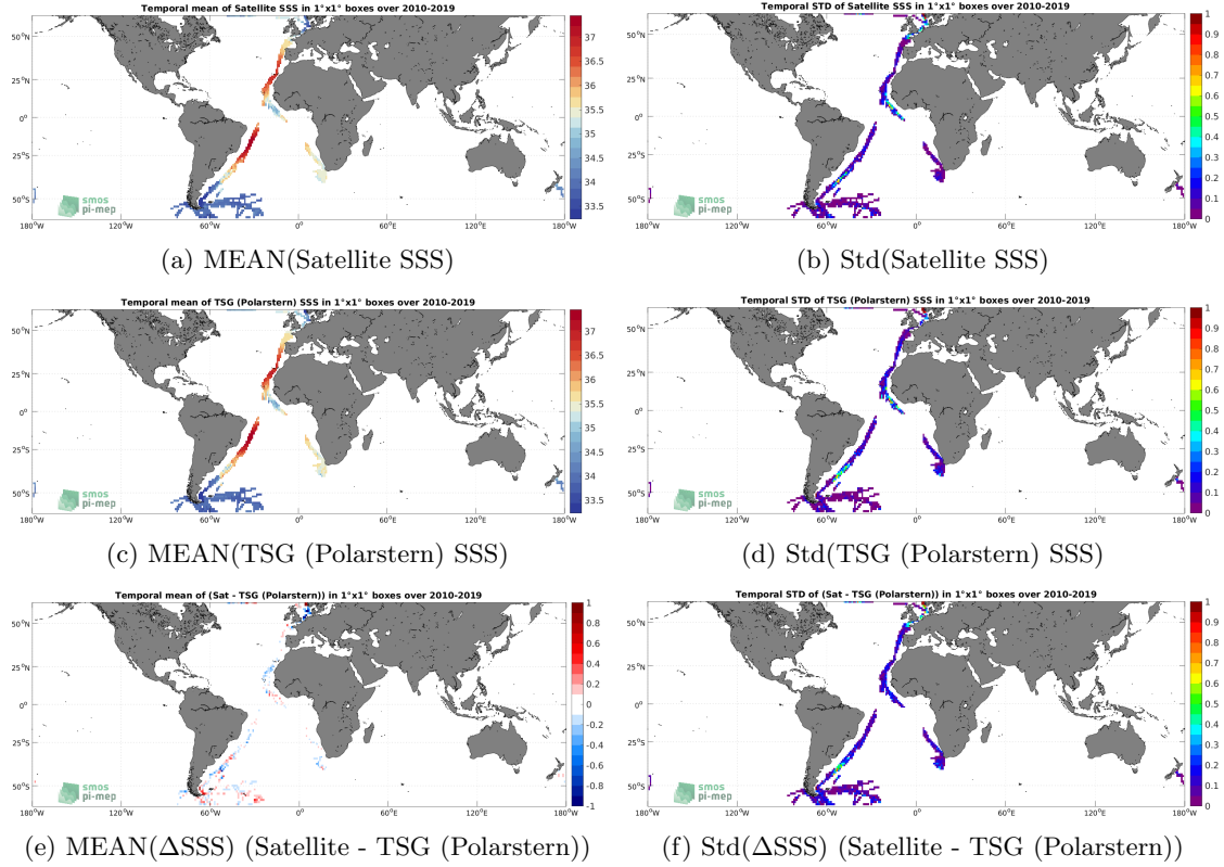
Figure 6: Temporal mean (left) and Std (right) of SSS from CCI SSS L4 Merged-OI v3.2 - 7-day running (ESA) (top), TSG (Polarstern) (middle), and of \Delta SSS (Satellite - TSG (Polarstern)). Only match-up pairs are used to generate these maps.
