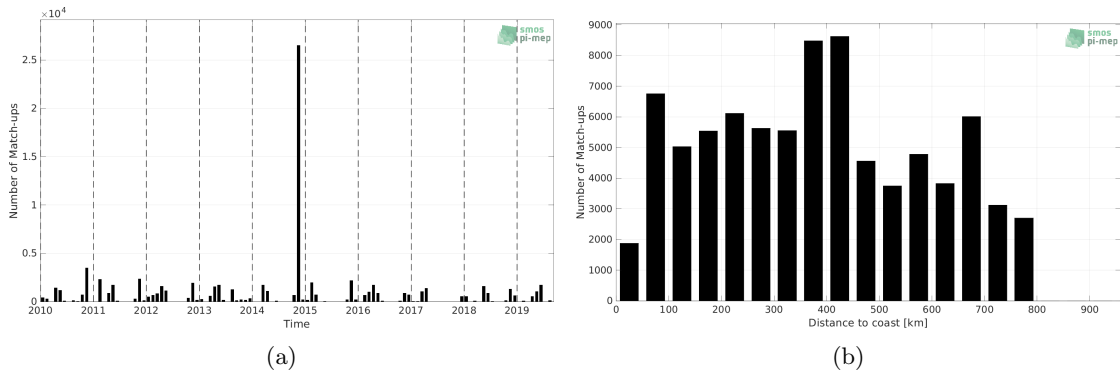
Figure 1: Number of match-ups between TSG (Polarstern) and CCI SSS L4 Merged-OI v3.2 - 7-day running (ESA) SSS as a function of time (a) and as function of the distance to coast (b) over the SMOS coastal zone (<800km) 60N-60S Pi-MEP region and for the full satellite product period.
