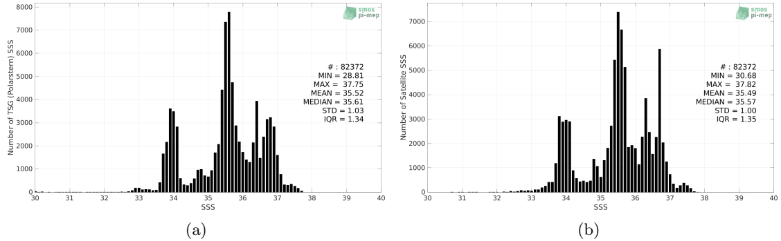
Figure 2: Histograms of SSS from TSG (Polarstern) (a) and CCI SSS L4 Merged-OI v3.2 - 7-day running (ESA) (b) considering all match-up pairs per bins of 0.1 over the SMOS coastal zone (<800km) 60N-60S Pi-MEP region and for the full satellite product period.
