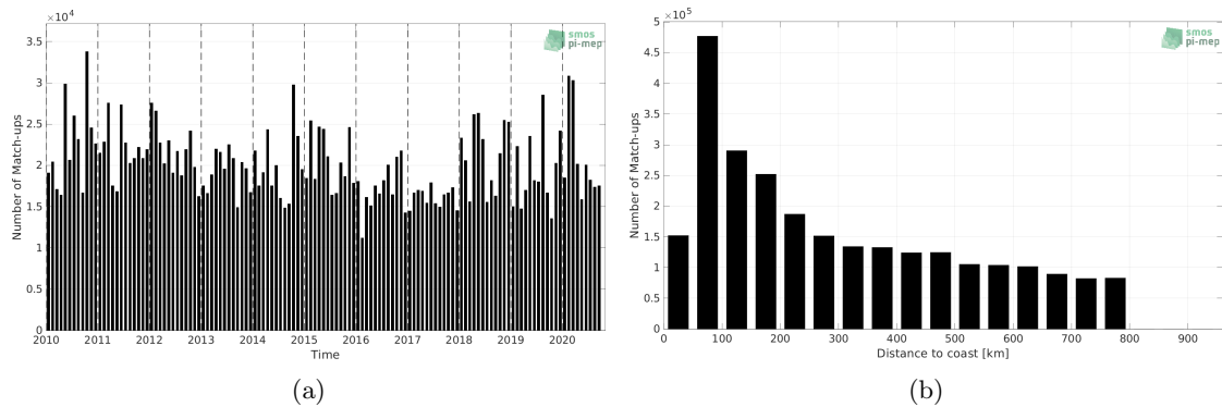
Figure 1: Number of match-ups between TSG (LEGOS-DM) and CCI SSS L4 Merged-OI v3.2 - 7-day running (ESA) SSS as a function of time (a) and as function of the distance to coast (b) over the SMOS coastal zone (<800km) 60N-60S Pi-MEP region and for the full satellite product period.
