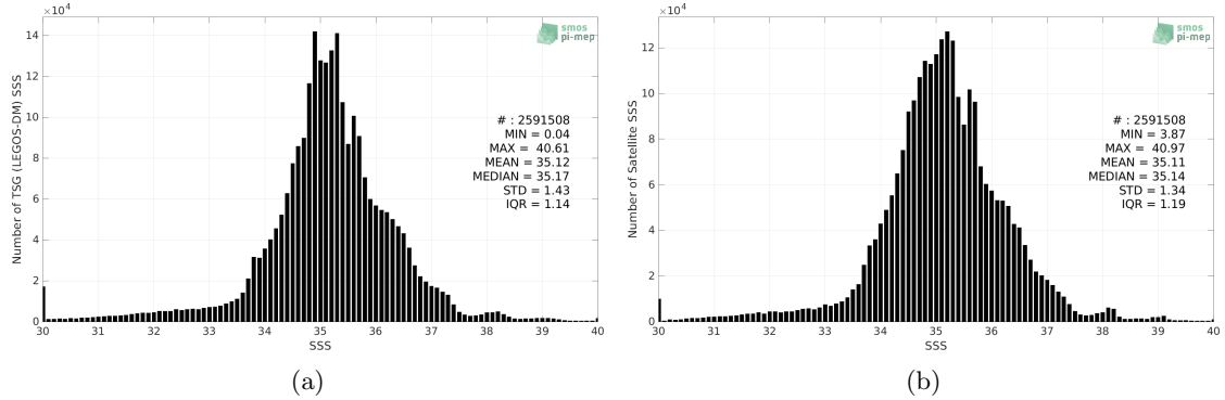
Figure 2: Histograms of SSS from TSG (LEGOS-DM) (a) and CCI SSS L4 Merged-OI v3.2 - 7-day running (ESA) (b) considering all match-up pairs per bins of 0.1 over the SMOS coastal zone (<800km) 60N-60S Pi-MEP region and for the full satellite product period.
