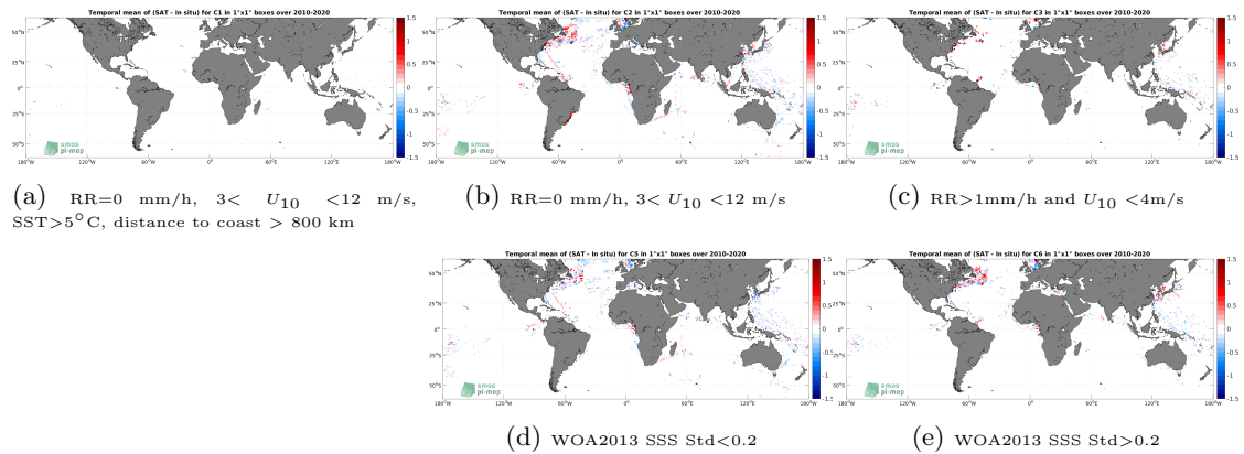
Figure 12: Temporal mean gridded over spatial boxes of size 1^\circ \times 1^\circ of \Delta SSS (CCI SSS L4 Merged-OI v3.2 - 7-day running (ESA) - TSG (LEGOS-DM)) for 5 different subdatasets corresponding to:RR=0 mm/h, 3 < U_{10} < 12 m/s, SST >5^\circ\text{C} , distance to coast > 800 km (a), RR=0 mm/h, 3 < U_{10} < 12 m/s (b), RR >1 mm/h and U_{10} < 4 m/s (c), WOA2013 SSS Std <0.2 (d), WOA2013 SSS Std >0.2 (e).
