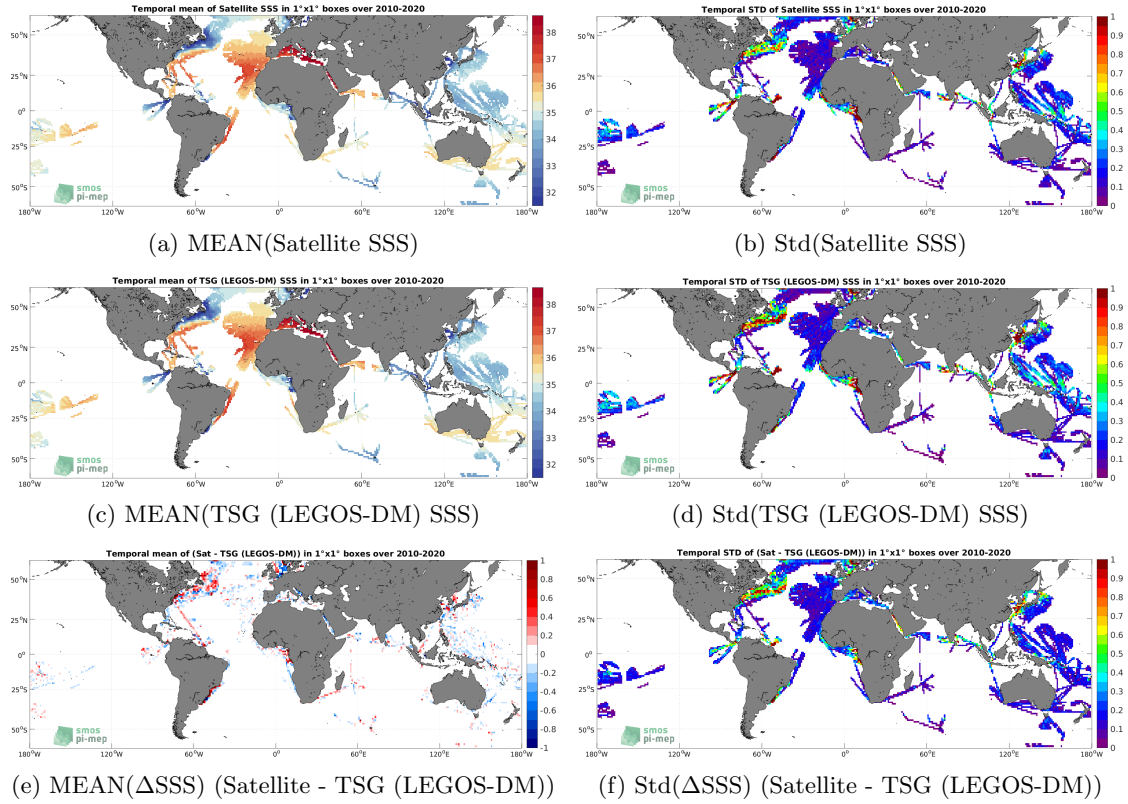
Figure 6: Temporal mean (left) and Std (right) of SSS from CCI SSS L4 Merged-OI v3.2 - 7-day running (ESA) (top), TSG (LEGOS-DM) (middle), and of \Delta SSS (Satellite - TSG (LEGOS-DM)). Only match-up pairs are used to generate these maps.
