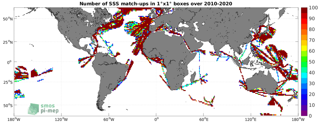
Figure 4: Number of SSS match-ups between TSG (LEGOS-DM) SSS and the CCI SSS L4 Merged-OI v3.2 - 7-day running (ESA) SSS product for the SMOS coastal zone (<800km) 60N-60S Pi-MEP region over 1^{\circ} \times 1^{\circ} boxes and for the full satellite product period.
