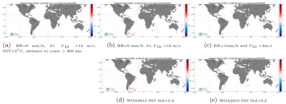
Figure 12: Temporal mean gridded over spatial boxes of size 1^\circ \times 1^\circ of \Delta\text{SSS} (CCI SSS L4 Merged-OI v3.2 - 7-day running (ESA) - TSG (GOSUD-Sailing-ship)) for 5 different subdatasets corresponding to: RR=0 mm/h, 3 < U_{10} < 12 m/s, SST > 5°C, distance to coast > 800 km (a), RR=0 mm/h, 3 < U_{10} < 12 m/s (b), RR > 1mm/h and U_{10} < 4 m/s (c), WOA2013 SSS Std < 0.2 (d), WOA2013 SSS Std > 0.2 (e).
