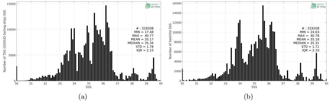
Figure 2: Histograms of SSS from TSG (GOSUD-Sailing-ship) (a) and CCI SSS L4 Merged-OI v3.2 - 7-day running (ESA) (b) considering all match-up pairs per bins of 0.1 over the SMOS coastal zone (<800km) 60N-60S Pi-MEP region and for the full satellite product period.
