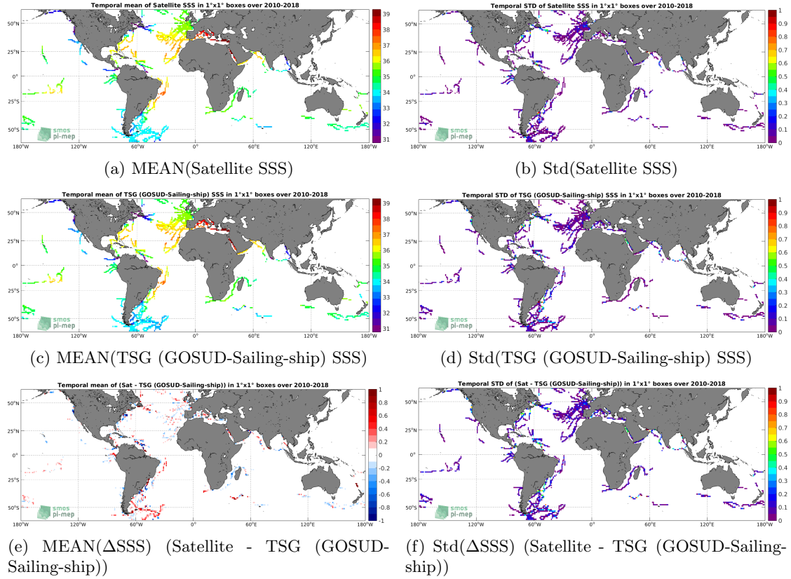
Figure 6: Temporal mean (left) and Std (right) of SSS from CCI SSS L4 Merged-OI v3.2 - 7-day running (ESA) (top), TSG (GOSUD-Sailing-ship) (middle), and of \Delta SSS (Satellite - TSG (GOSUD-Sailing-ship)). Only match-up pairs are used to generate these maps.
