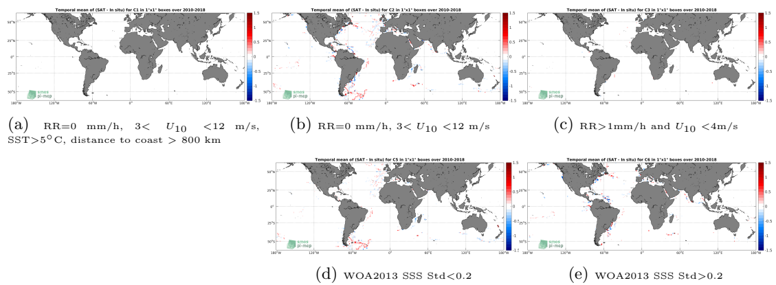
Figure 12: Temporal mean gridded over spatial boxes of size 1°x1° of \Delta SSS (CCI SSS L4 Merged-OI v3.2 - 7-day running (ESA) - TSG (GOSUD-Sailing-ship)) for 5 different subdatasets corresponding to:RR=0 mm/h, 3 < U_{10} < 12 m/s, SST>5°C, distance to coast > 800 km (a), RR=0 mm/h, 3 < U_{10} < 12 m/s (b), RR>1mm/h and U_{10} < 4 m/s (c), WOA2013 SSS Std<0.2 (d), WOA2013 SSS Std>0.2 (e).
