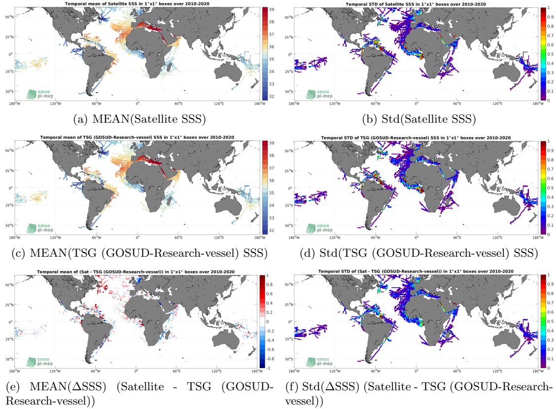
Figure 6: Temporal mean (left) and Std (right) of SSS from CCI SSS L4 Merged-OI v3.2 - 7-day running (ESA) (top), TSG (GOSUD-Research-vessel) (middle), and of \Delta\text{SSS} (Satellite - TSG (GOSUD-Research-vessel)). Only match-up pairs are used to generate these maps.
