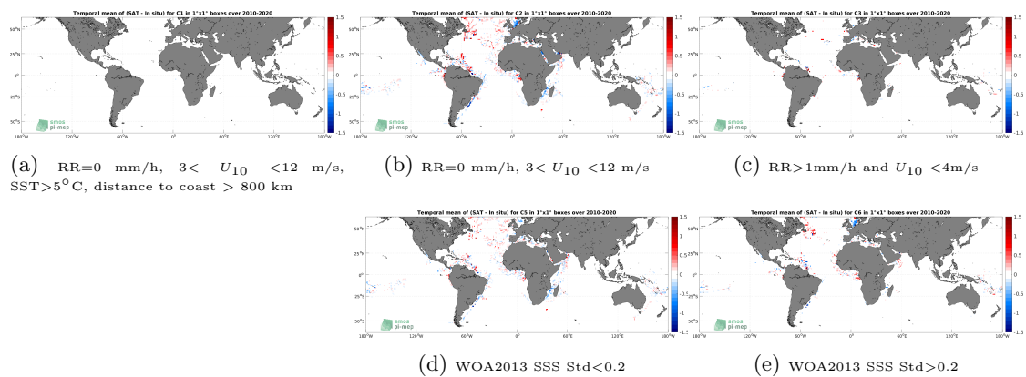
Figure 12: Temporal mean gridded over spatial boxes of size 1^\circ \times 1^\circ of \Delta SSS (CCI SSS L4 Merged-OI v3.2 - 7-day running (ESA) - TSG (GOSUD-Research-vessel)) for 5 different subdatasets corresponding to:RR=0 mm/h, 3 < U_{10} < 12 m/s, SST >5^\circ C, distance to coast > 800 km (a), RR=0 mm/h, 3 < U_{10} < 12 m/s (b), RR >1 mm/h and U_{10} < 4 m/s (c), WOA2013 SSS Std <0.2 (d), WOA2013 SSS Std >0.2 (e).
