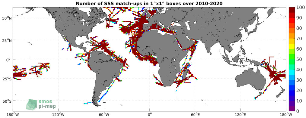
Figure 4: Number of SSS match-ups between TSG (GOSUD-Research-vessel) SSS and the CCI SSS L4 Merged-OI v3.2 - 7-day running (ESA) SSS product for the SMOS coastal zone (<800km) 60N-60S Pi-MEP region over 1^\circ \times 1^\circ boxes and for the full satellite product period.
