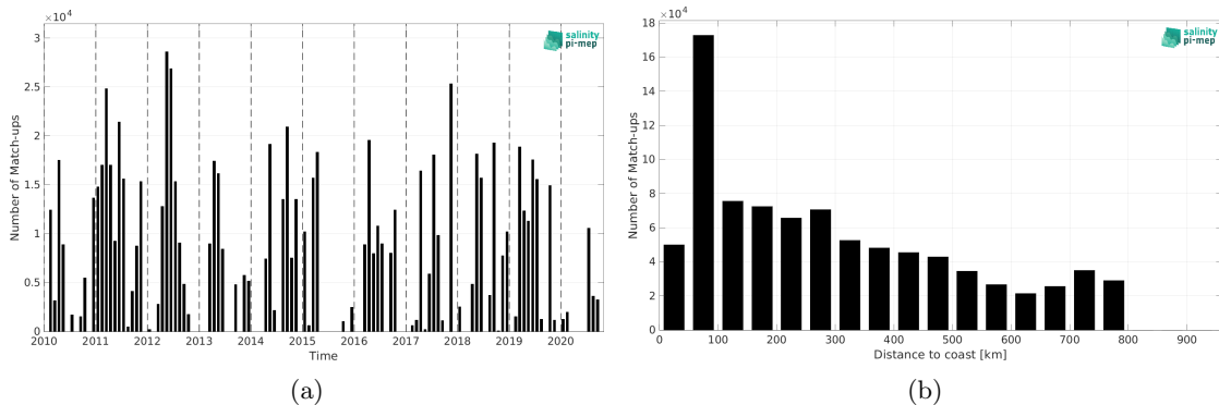
Figure 1: Number of match-ups between TSG (CSIC-UTM) and CCI SSS L4 Merged-OI v3.2 - 7-day running (ESA) SSS as a function of time (a) and as function of the distance to coast (b) over the SMOS coastal zone (<800km) 60N-60S Pi-MEP region and for the full satellite product period.
