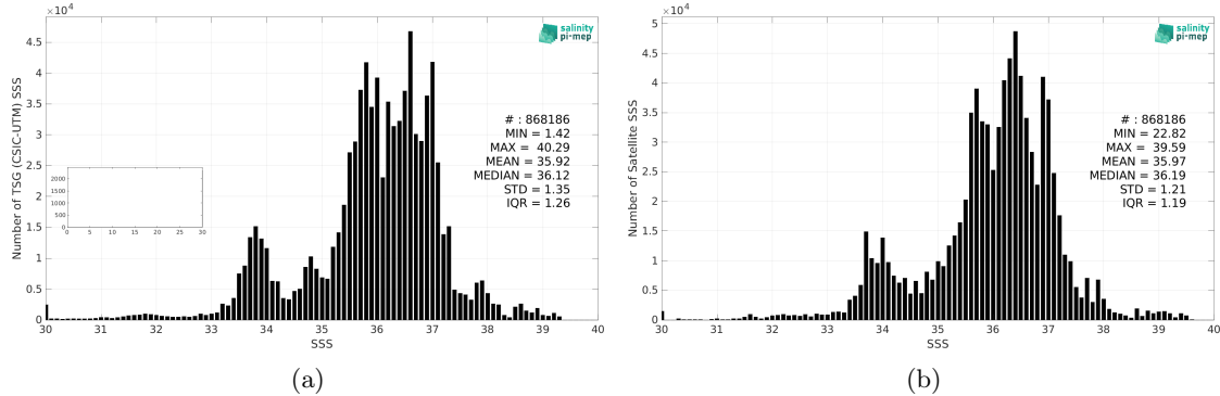
Figure 2: Histograms of SSS from TSG (CSIC-UTM) (a) and CCI SSS L4 Merged-OI v3.2 - 7-day running (ESA) (b) considering all match-up pairs per bins of 0.1 over the SMOS coastal zone (<800km) 60N-60S Pi-MEP region and for the full satellite product period.
