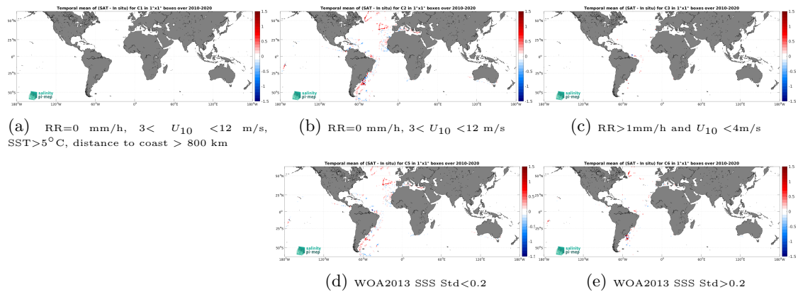
Figure 12: Temporal mean gridded over spatial boxes of size 1^\circ \times 1^\circ of \Delta SSS (CCI SSS L4 Merged-OI v3.2 - 7-day running (ESA) - TSG (CSIC-UTM)) for 5 different subdatasets corresponding to:RR=0 mm/h, 3 < U_{10} < 12 m/s, SST >5^\circ C, distance to coast > 800 km (a), RR=0 mm/h, 3 < U_{10} < 12 m/s (b), RR >1 mm/h and U_{10} < 4 m/s (c), WOA2013 SSS Std <0.2 (d), WOA2013 SSS Std >0.2 (e).
