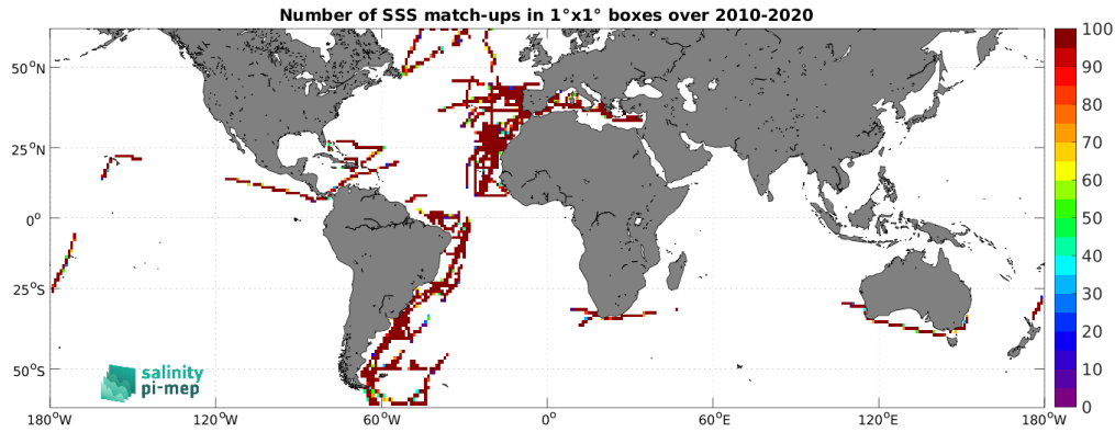
Figure 4: Number of SSS match-ups between TSG (CSIC-UTM) SSS and the CCI SSS L4 Merged-OI v3.2 - 7-day running (ESA) SSS product for the SMOS coastal zone (<800km) 60N-60S Pi-MEP region over 1^\circ \times 1^\circ boxes and for the full satellite product period.
