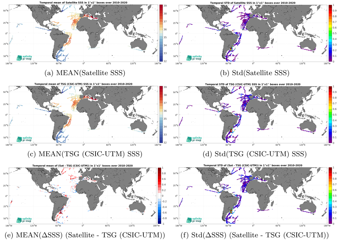
Figure 6: Temporal mean (left) and Std (right) of SSS from CCI SSS L4 Merged-OI v3.2 - 7-day running (ESA) (top), TSG (CSIC-UTM) (middle), and of \Delta SSS (Satellite - TSG (CSIC-UTM)). Only match-up pairs are used to generate these maps.
