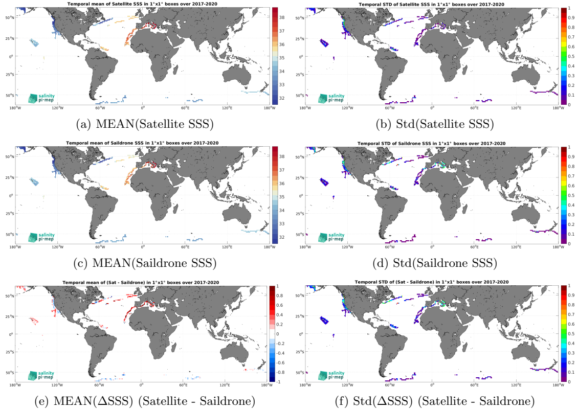
Figure 6: Temporal mean (left) and Std (right) of SSS from CCI SSS L4 Merged-OI v3.2 - 7-day running (ESA) (top), Saildrone (middle), and of \Delta SSS (Satellite - Saildrone). Only match-up pairs are used to generate these maps.
