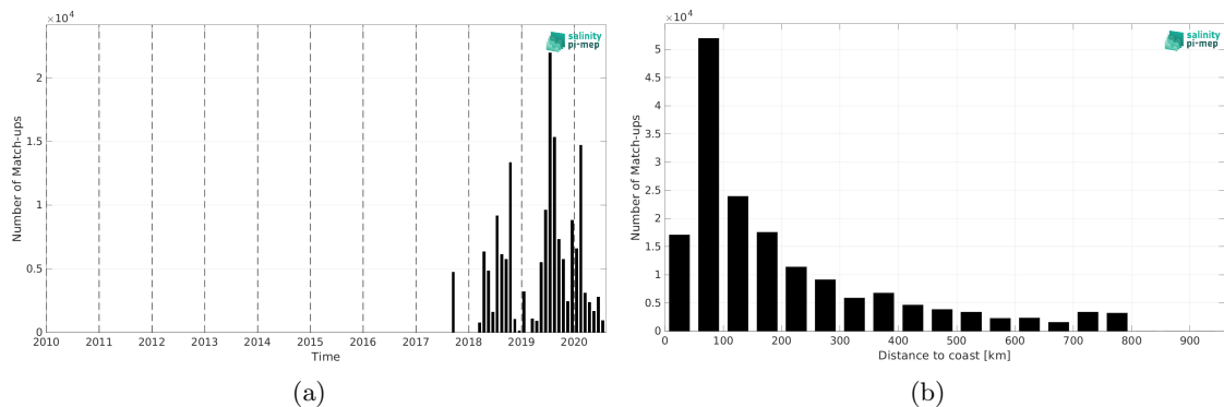
Figure 1: Number of match-ups between Saildrone and CCI SSS L4 Merged-OI v3.2 - 7-day running (ESA) SSS as a function of time (a) and as function of the distance to coast (b) over the SMOS coastal zone (<800km) 60N-60S Pi-MEP region and for the full satellite product period.
