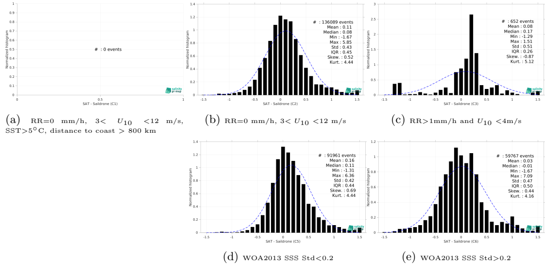
Figure 13: Normalized histogram of \Delta SSS (CCI SSS L4 Merged-OI v3.2 - 7-day running (ESA) - Saiddrone) for 5 different subdatasets corresponding to: RR=0 mm/h, 3 < U_{10} < 12 m/s, SST > 5°C, distance to coast > 800 km (a), RR=0 mm/h, 3 < U_{10} < 12 m/s (b), RR > 1mm/h and U_{10} < 4 m/s (c), WOA2013 SSS Std < 0.2 (d), WOA2013 SSS Std > 0.2 (e).
