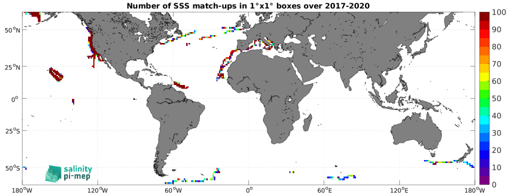
Figure 4: Number of SSS match-ups between Saildrone SSS and the CCI SSS L4 Merged-OI v3.2 - 7-day running (ESA) SSS product for the SMOS coastal zone ( <800\text{km} ) 60N-60S Pi-MEP region over 1^\circ \times 1^\circ boxes and for the full satellite product period.
