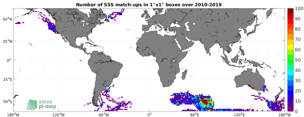
Figure 4: Number of SSS match-ups between Marine mammals SSS and the CCI SSS L4 Merged-OI v3.2 - 7-day running (ESA) SSS product for the SMOS coastal zone (<800km) 60N-60S Pi-MEP region over 1^\circ \times 1^\circ boxes and for the full satellite product period.
