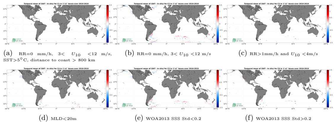
Figure 12: Temporal mean gridded over spatial boxes of size 1^\circ \times 1^\circ of \Delta SSS (CCI SSS L4 Merged-OI v3.2 - 7-day running (ESA) - Marine mammals) for 6 different subdatasets corresponding to: RR=0 mm/h, 3 < U_{10} < 12 m/s, SST > 5^\circ C, distance to coast > 800 km (a), RR=0 mm/h, 3 < U_{10} < 12 m/s (b), RR > 1 mm/h and U_{10} < 4 m/s (c),MLD < 20 m (d),WOA2013 SSS Std < 0.2 (e),WOA2013 SSS Std > 0.2 (f).
