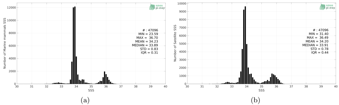
Figure 2: Histograms of SSS from Marine mammals (a) and CCI SSS L4 Merged-OI v3.2 - 7-day running (ESA) (b) considering all match-up pairs per bins of 0.1 over the SMOS coastal zone (<800km) 60N-60S Pi-MEP region and for the full satellite product period.
