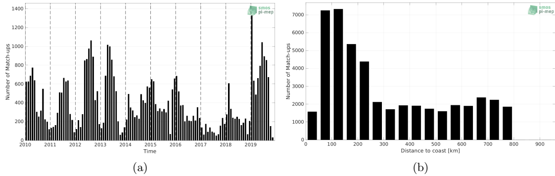
Figure 1: Number of match-ups between Marine mammals and CCI SSS L4 Merged-OI v3.2 - 7-day running (ESA) SSS as a function of time (a) and as function of the distance to coast (b) over the SMOS coastal zone (<800km) 60N-60S Pi-MEP region and for the full satellite product period.
