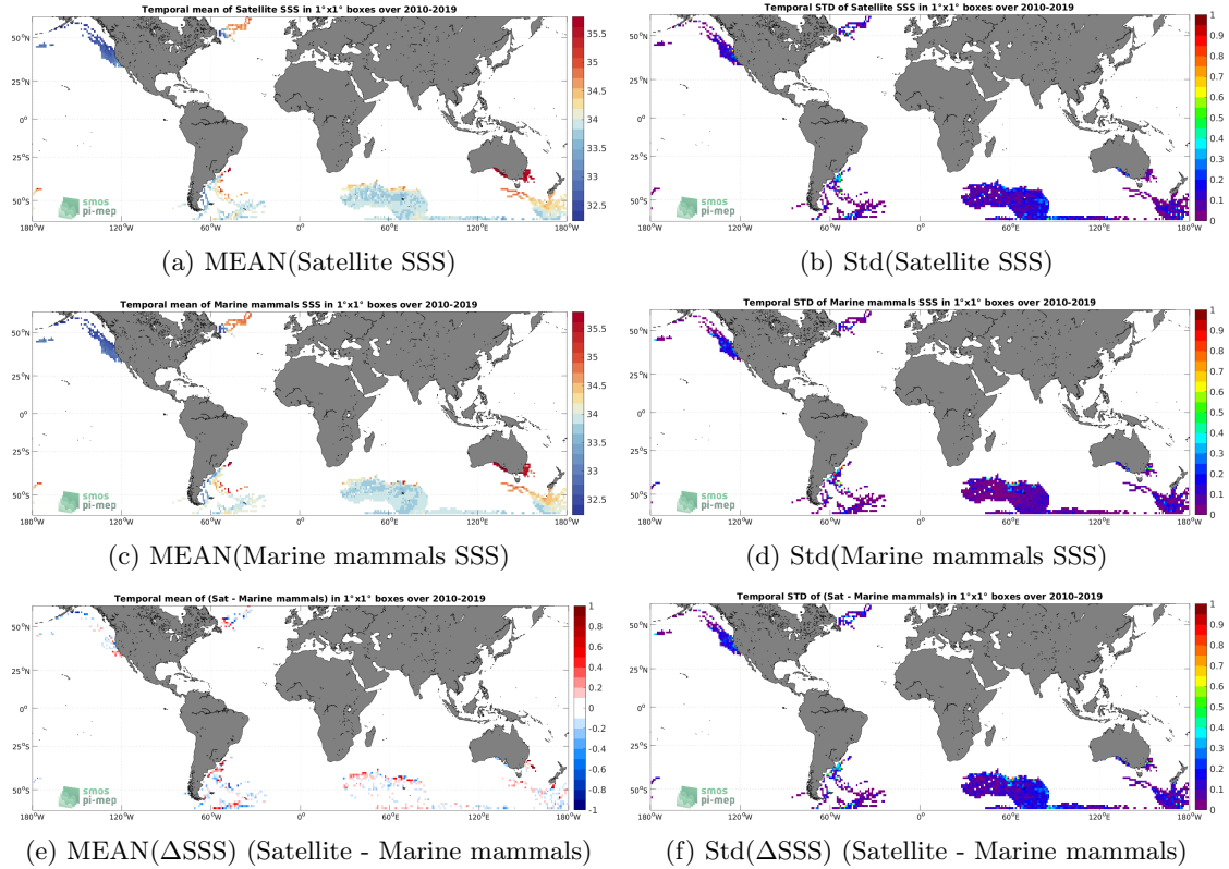
Figure 6: Temporal mean (left) and Std (right) of SSS from CCI SSS L4 Merged-OI v3.2 - 7-day running (ESA) (top), Marine mammals (middle), and of \Delta SSS (Satellite - Marine mammals). Only match-up pairs are used to generate these maps.
