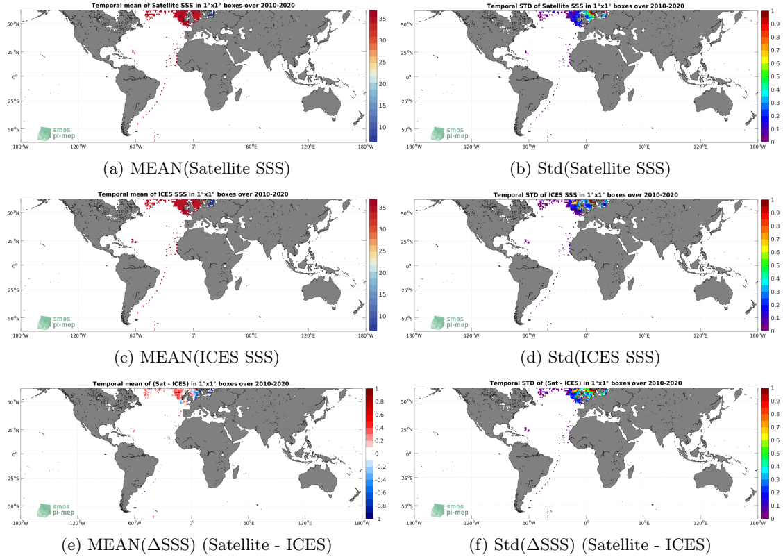
Figure 6: Temporal mean (left) and Std (right) of SSS from CCI SSS L4 Merged-OI v3.2 - 7-day running (ESA) (top), ICES (middle), and of \Delta SSS (Satellite - ICES). Only match-up pairs are used to generate these maps.
