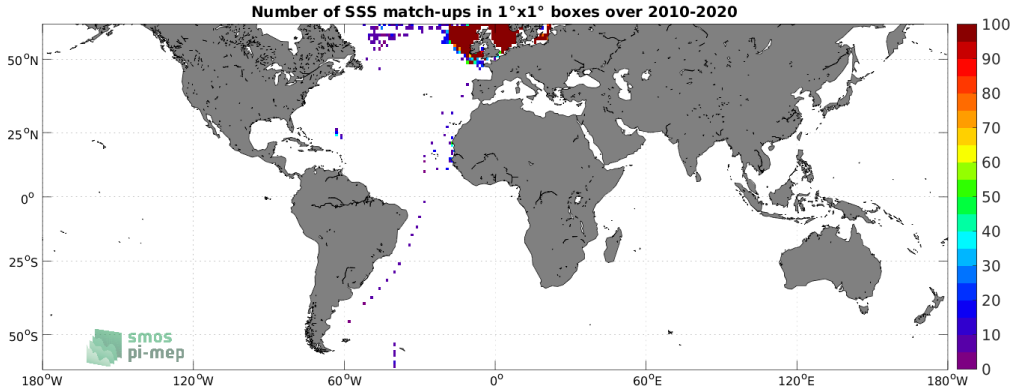
Figure 4: Number of SSS match-ups between ICES SSS and the CCI SSS L4 Merged-OI v3.2 - 7-day running (ESA) SSS product for the SMOS coastal zone (<800km) 60N-60S Pi-MEP region over 1^\circ \times 1^\circ boxes and for the full satellite product period.
