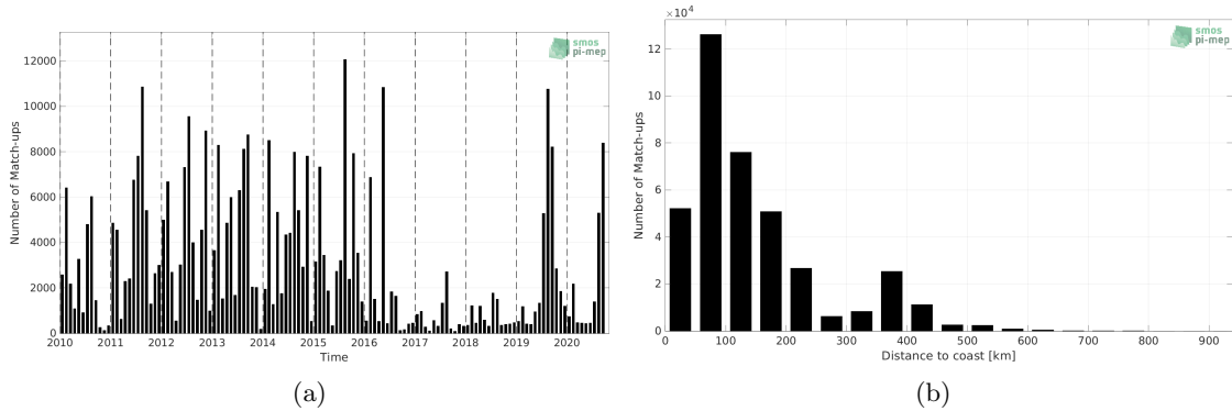
Figure 1: Number of match-ups between ICES and CCI SSS L4 Merged-OI v3.2 - 7-day running (ESA) SSS as a function of time (a) and as function of the distance to coast (b) over the SMOS coastal zone (<800km) 60N-60S Pi-MEP region and for the full satellite product period.
