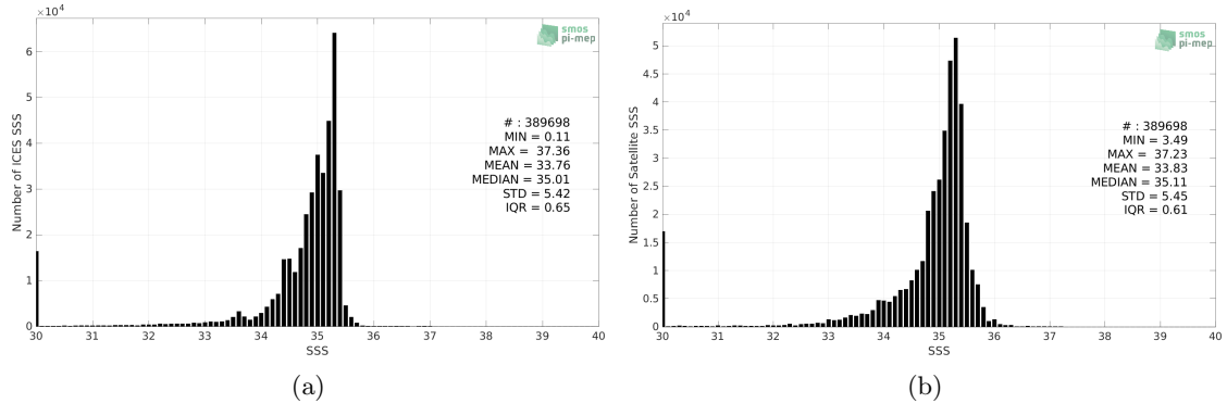
Figure 2: Histograms of SSS from ICES (a) and CCI SSS L4 Merged-OI v3.2 - 7-day running (ESA) (b) considering all match-up pairs per bins of 0.1 over the SMOS coastal zone (<800km) 60N-60S Pi-MEP region and for the full satellite product period.
