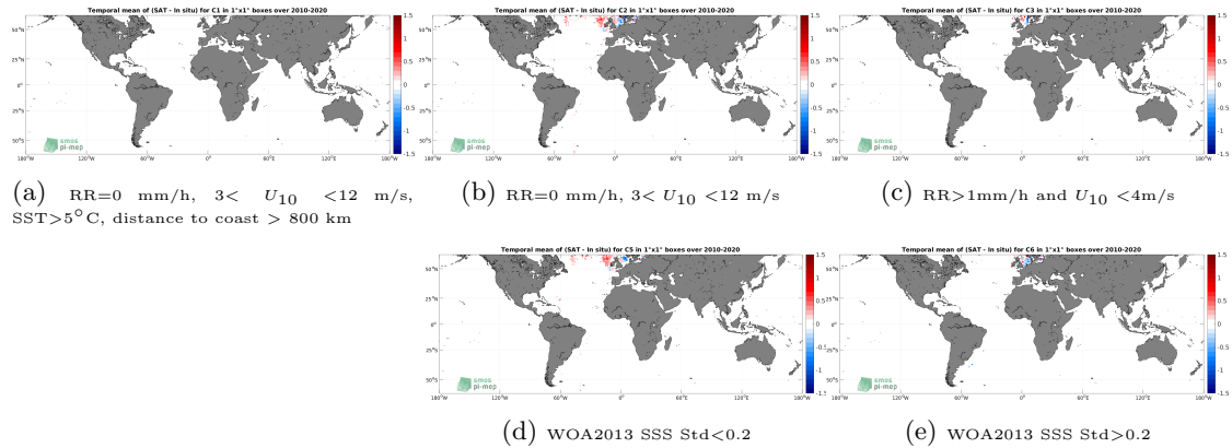
Figure 12: Temporal mean gridded over spatial boxes of size 1^\circ \times 1^\circ of \Delta SSS (CCI SSS L4 Merged-OI v3.2 - 7-day running (ESA) - ICES) for 5 different subdatasets corresponding to:RR=0 mm/h, 3 < U_{10} < 12 m/s, SST >5^\circ\text{C} , distance to coast > 800 km (a), RR=0 mm/h, 3 < U_{10} < 12 m/s (b), RR >1 mm/h and U_{10} < 4 m/s (c), WOA2013 SSS Std <0.2 (d), WOA2013 SSS Std >0.2 (e).
