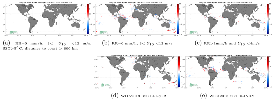
Figure 11: Temporal mean gridded over spatial boxes of size 1^\circ \times 1^\circ of \Delta SSS (CCI SSS L4 Merged-OI v3.2 - 7-day running (ESA) - Surface drifters) for 5 different subdatasets corresponding to:RR=0 mm/h, 3 < U_{10} < 12 m/s, SST >5^\circ C, distance to coast > 800 km (a), RR=0 mm/h, 3 < U_{10} < 12 m/s (b), RR >1 mm/h and U_{10} < 4 m/s (c), WOA2013 SSS Std <0.2 (d), WOA2013 SSS Std >0.2 (e).
