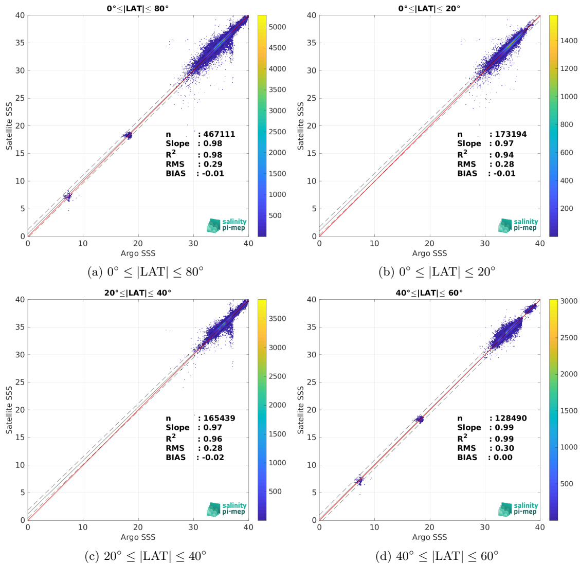
Figure 9: Contour maps of the concentration of CCI SSS L4 Merged-OI v3.2 - 7-day running (ESA) SSS (y-axis) versus Argo SSS (x-axis) at match-up pairs for different latitude bands. For each plot, the red line shows x=y . The black thin and dashed lines indicate a linear fit through the data cloud and the \pm 95\% confidence levels, respectively. The number match-up pairs n , the slope and R^2 coefficient of the linear fit, the root mean square (RMS) and the mean bias between satellite and in situ data are indicated for each latitude band in each plot.
