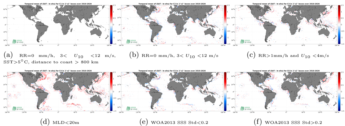
Figure 12: Temporal mean gridded over spatial boxes of size 1^\circ \times 1^\circ of \Delta SSS (CCI SSS L4 Merged-OI v3.2 - 7-day running (ESA) - Argo) for 6 different subdatasets corresponding to:RR=0 mm/h, 3 < U_{10} < 12 m/s, SST >5^\circ C, distance to coast > 800 km (a), RR=0 mm/h, 3 < U_{10} < 12 m/s (b), RR >1 mm/h and U_{10} < 4 m/s (c),MLD <20 m (d),WOA2013 SSS Std <0.2 (e),WOA2013 SSS Std >0.2 (f).
