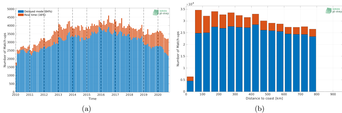
Figure 1: Number of match-ups between Argo and CCI SSS L4 Merged-OI v3.2 - 7-day running (ESA) SSS as a function of time (a) and as function of the distance to coast (b) over the SMOS coastal zone (<800km) 60N-60S Pi-MEP region and for the full satellite product period.
