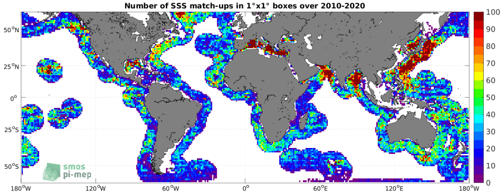
Figure 4: Number of SSS match-ups between Argo SSS and the CCI SSS L4 Merged-OI v3.2 - 7-day running (ESA) SSS product for the SMOS coastal zone (<800km) 60N-60S Pi-MEP region over 1^\circ \times 1^\circ boxes and for the full satellite product period.
