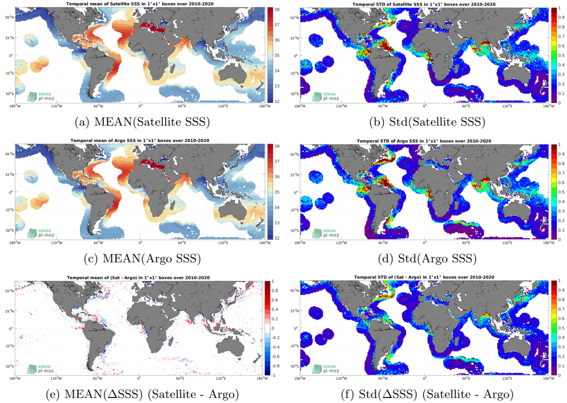
Figure 6: Temporal mean (left) and Std (right) of SSS from CCI SSS L4 Merged-OI v3.2 - 7-day running (ESA) (top), Argo (middle), and of \Delta SSS (Satellite - Argo). Only match-up pairs are used to generate these maps.
