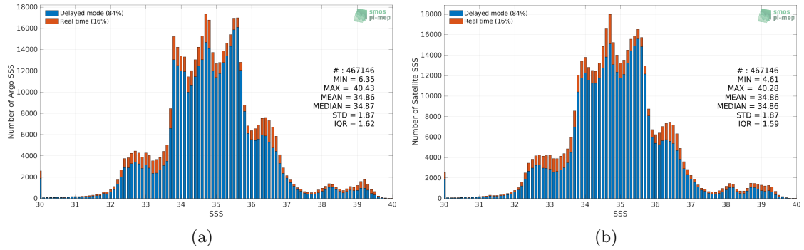
Figure 2: Histograms of SSS from Argo (a) and CCI SSS L4 Merged-OI v3.2 - 7-day running (ESA) (b) considering all match-up pairs per bins of 0.1 over the SMOS coastal zone (<800km) 60N-60S Pi-MEP region and for the full satellite product period.
