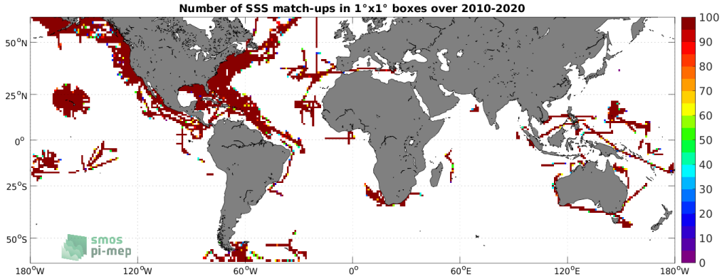
Figure 4: Number of SSS match-ups between TSG (SAMOS) SSS and the CCI SSS L4 Merged-OI v3.2 - 30-day running (ESA) SSS product for the SMOS coastal zone (<800km) 60N-60S Pi-MEP region over 1^\circ \times 1^\circ boxes and for the full satellite product period.
