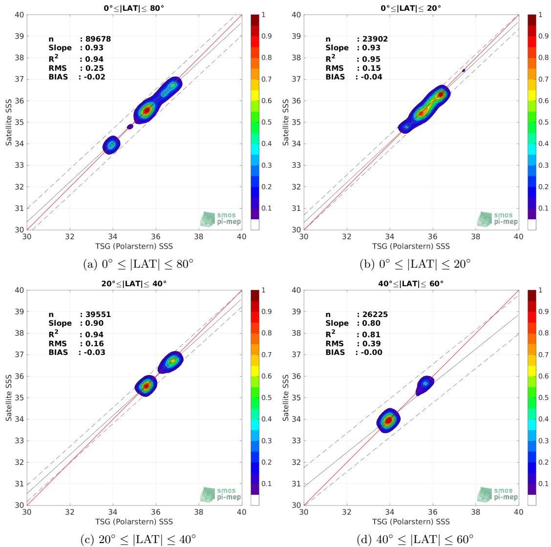
Figure 9: Contour maps of the concentration of CCI SSS L4 Merged-OI v3.2 - 30-day running (ESA) SSS (y-axis) versus TSG (Polarstern) SSS (x-axis) at match-up pairs for different latitude bands. For each plot, the red line shows x=y . The black thin and dashed lines indicate a linear fit through the data cloud and the \pm 95\% confidence levels, respectively. The number match-up pairs n , the slope and R^2 coefficient of the linear fit, the root mean square (RMS) and the mean bias between satellite and in situ data are indicated for each latitude band in each plots.
