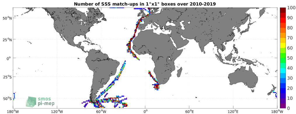
Figure 4: Number of SSS match-ups between TSG (Polarstern) SSS and the CCI SSS L4 Merged-OI v3.2 - 30-day running (ESA) SSS product for the SMOS coastal zone (<800km) 60N-60S Pi-MEP region over 1^\circ \times 1^\circ boxes and for the full satellite product period.
