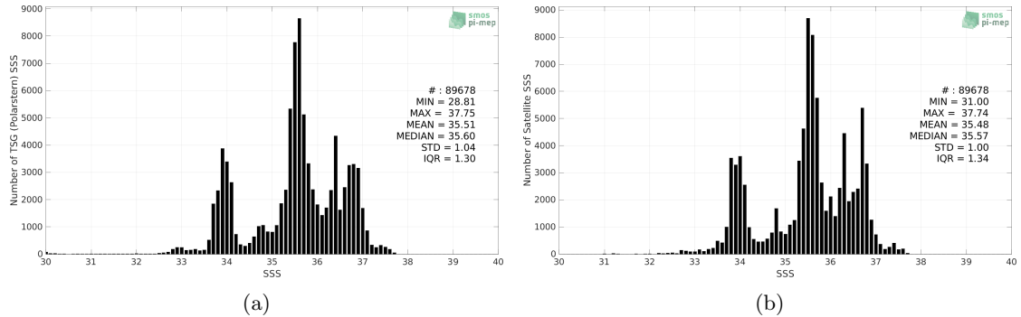
Figure 2: Histograms of SSS from TSG (Polarstern) (a) and CCI SSS L4 Merged-OI v3.2 - 30-day running (ESA) (b) considering all match-up pairs per bins of 0.1 over the SMOS coastal zone (<800km) 60N-60S Pi-MEP region and for the full satellite product period.
