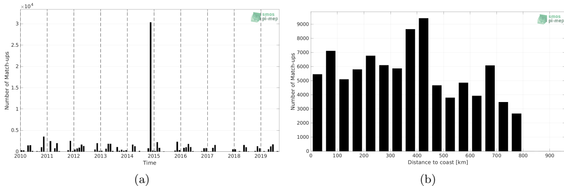
Figure 1: Number of match-ups between TSG (Polarstern) and CCI SSS L4 Merged-OI v3.2 - 30-day running (ESA) SSS as a function of time (a) and as function of the distance to coast (b) over the SMOS coastal zone (<800km) 60N-60S Pi-MEP region and for the full satellite product period.
