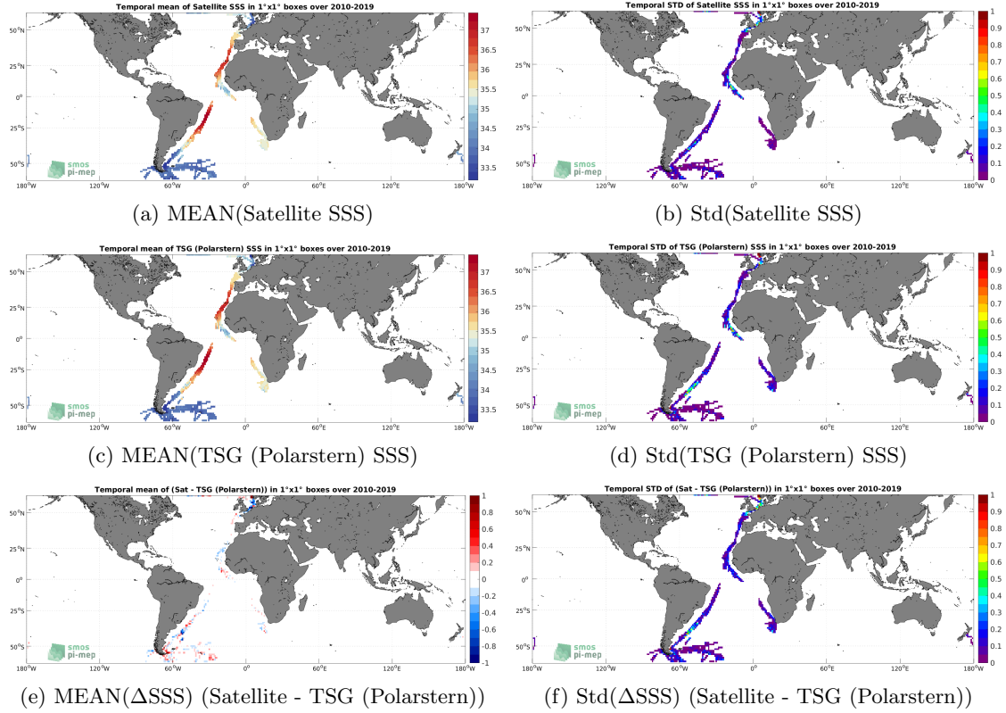
Figure 6: Temporal mean (left) and Std (right) of SSS from CCI SSS L4 Merged-OI v3.2 - 30-day running (ESA) (top), TSG (Polarstern) (middle), and of \Delta SSS (Satellite - TSG (Polarstern)). Only match-up pairs are used to generate these maps.
