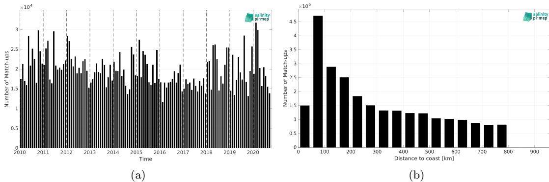
Figure 1: Number of match-ups between TSG (LEGOS-DM) and CCI SSS L4 Merged-OI v3.2 - 30-day running (ESA) SSS as a function of time (a) and as function of the distance to coast (b) over the SMOS coastal zone (<800km) 60N-60S Pi-MEP region and for the full satellite product period.
