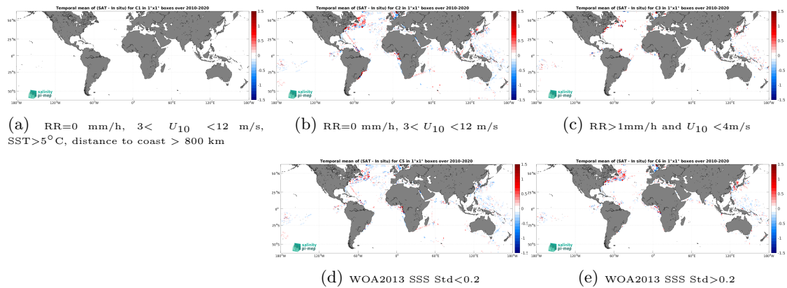
Figure 12: Temporal mean gridded over spatial boxes of size 1^\circ \times 1^\circ of \Delta\text{SSS} (CCI SSS L4 Merged-OI v3.2 - 30-day running (ESA) - TSG (LEGOS-DM)) for 5 different subdatasets corresponding to:RR=0 mm/h, 3 < U_{10} < 12 m/s, SST >5^\circ\text{C} , distance to coast > 800 km (a), RR=0 mm/h, 3 < U_{10} < 12 m/s (b), RR >1 mm/h and U_{10} < 4 m/s (c), WOA2013 SSS Std <0.2 (d), WOA2013 SSS Std >0.2 (e).
