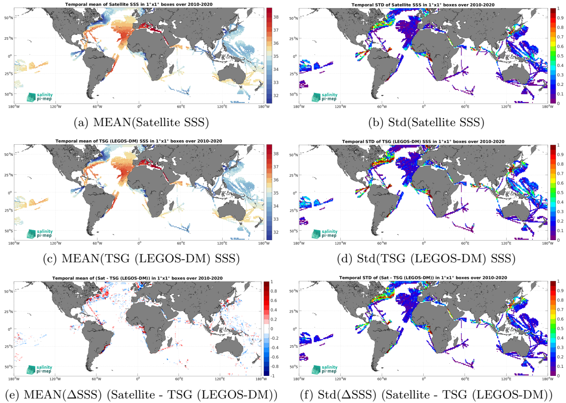
Figure 6: Temporal mean (left) and Std (right) of SSS from CCI SSS L4 Merged-OI v3.2 - 30-day running (ESA) (top), TSG (LEGOS-DM) ( in situ ) dataset (middle), and of \Delta SSS (Satellite - TSG (LEGOS-DM)). Only match-up pairs are used to generate these maps.
