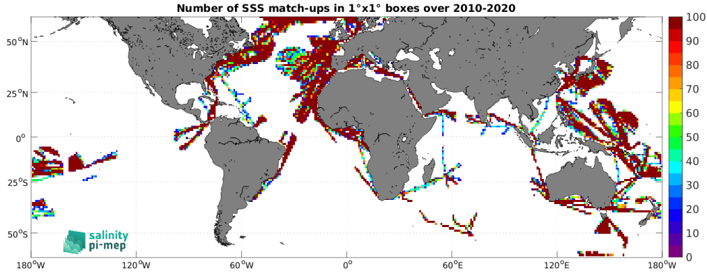
Figure 4: Number of SSS match-ups between TSG (LEGOS-DM) SSS and the CCI SSS L4 Merged-OI v3.2 - 30-day running (ESA) SSS product for the SMOS coastal zone (<800km) 60N-60S Pi-MEP region over 1^{\circ} \times 1^{\circ} boxes and for the full satellite product period.
