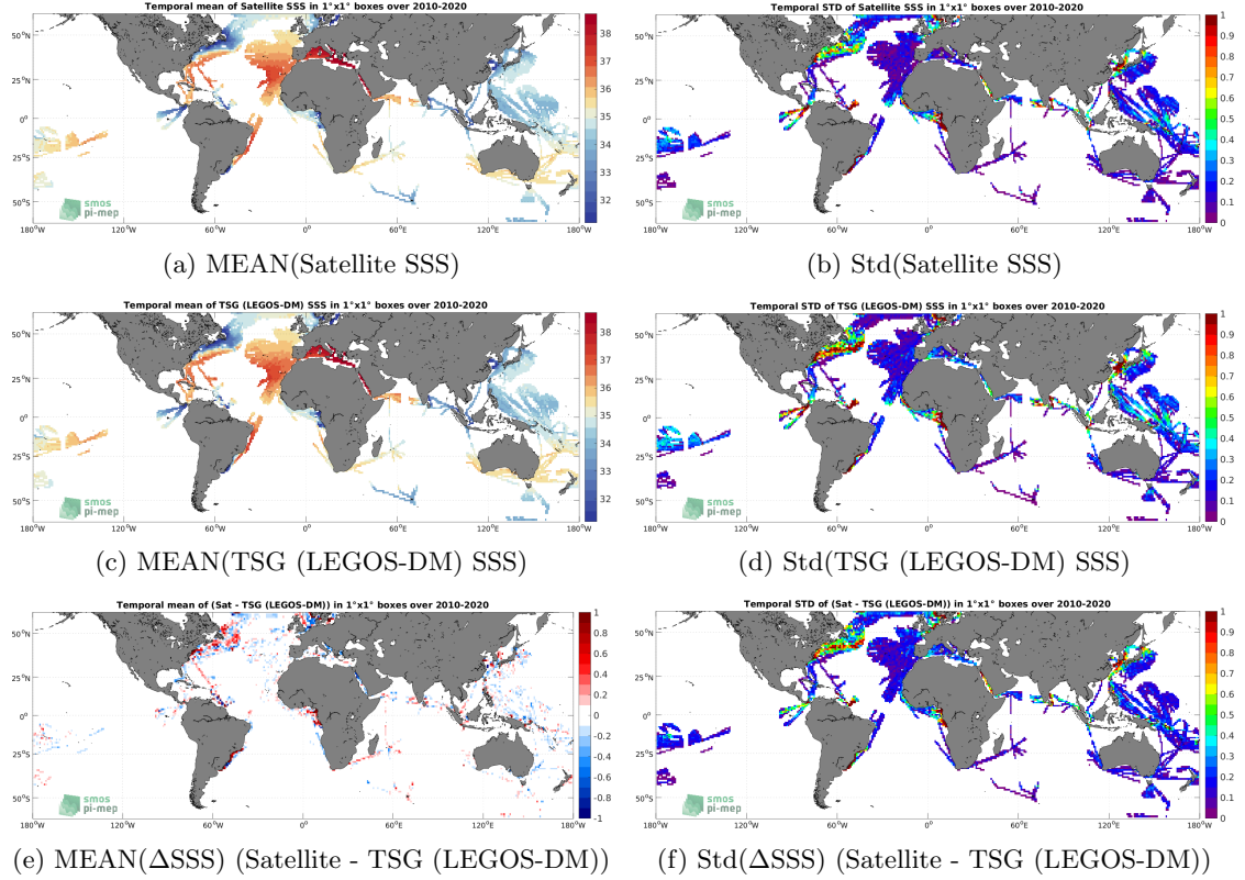
Figure 6: Temporal mean (left) and Std (right) of SSS from CCI SSS L4 Merged-OI v3.2 - 30-day running (ESA) (top), TSG (LEGOS-DM) (middle), and of \Delta SSS (Satellite - TSG (LEGOS-DM)). Only match-up pairs are used to generate these maps.
