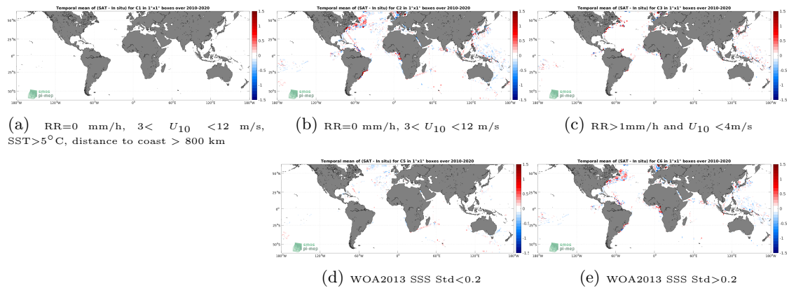
Figure 12: Temporal mean gridded over spatial boxes of size 1^\circ \times 1^\circ of \Delta SSS (CCI SSS L4 Merged-OI v3.2 - 30-day running (ESA) - TSG (LEGOS-DM)) for 5 different subdatasets corresponding to:RR=0 mm/h, 3 < U_{10} < 12 m/s, SST >5^\circ\text{C} , distance to coast > 800 km (a), RR=0 mm/h, 3 < U_{10} < 12 m/s (b), RR >1 mm/h and U_{10} < 4 m/s (c), WOA2013 SSS Std <0.2 (d), WOA2013 SSS Std >0.2 (e).
