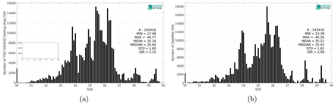
Figure 2: Histograms of SSS from TSG (GOSUD-Sailing-ship) (a) and CCI SSS L4 Merged-OI v3.2 - 30-day running (ESA) (b) considering all match-up pairs per bins of 0.1 over the SMOS coastal zone (<800km) 60N-60S Pi-MEP region and for the full satellite product period.
