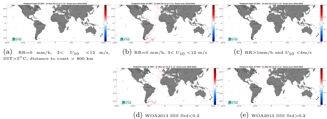
Figure 12: Temporal mean gridded over spatial boxes of size 1^\circ \times 1^\circ of \Delta\text{SSS} (CCI SSS L4 Merged-OI v3.2 - 30-day running (ESA) - TSG (GOSUD-Sailing-ship)) for 5 different subdatasets corresponding to: RR=0 mm/h, 3 < U_{10} < 12 m/s, SST > 5°C, distance to coast > 800 km (a), RR=0 mm/h, 3 < U_{10} < 12 m/s (b), RR > 1mm/h and U_{10} < 4 m/s (c), WOA2013 SSS Std < 0.2 (d), WOA2013 SSS Std > 0.2 (e).
