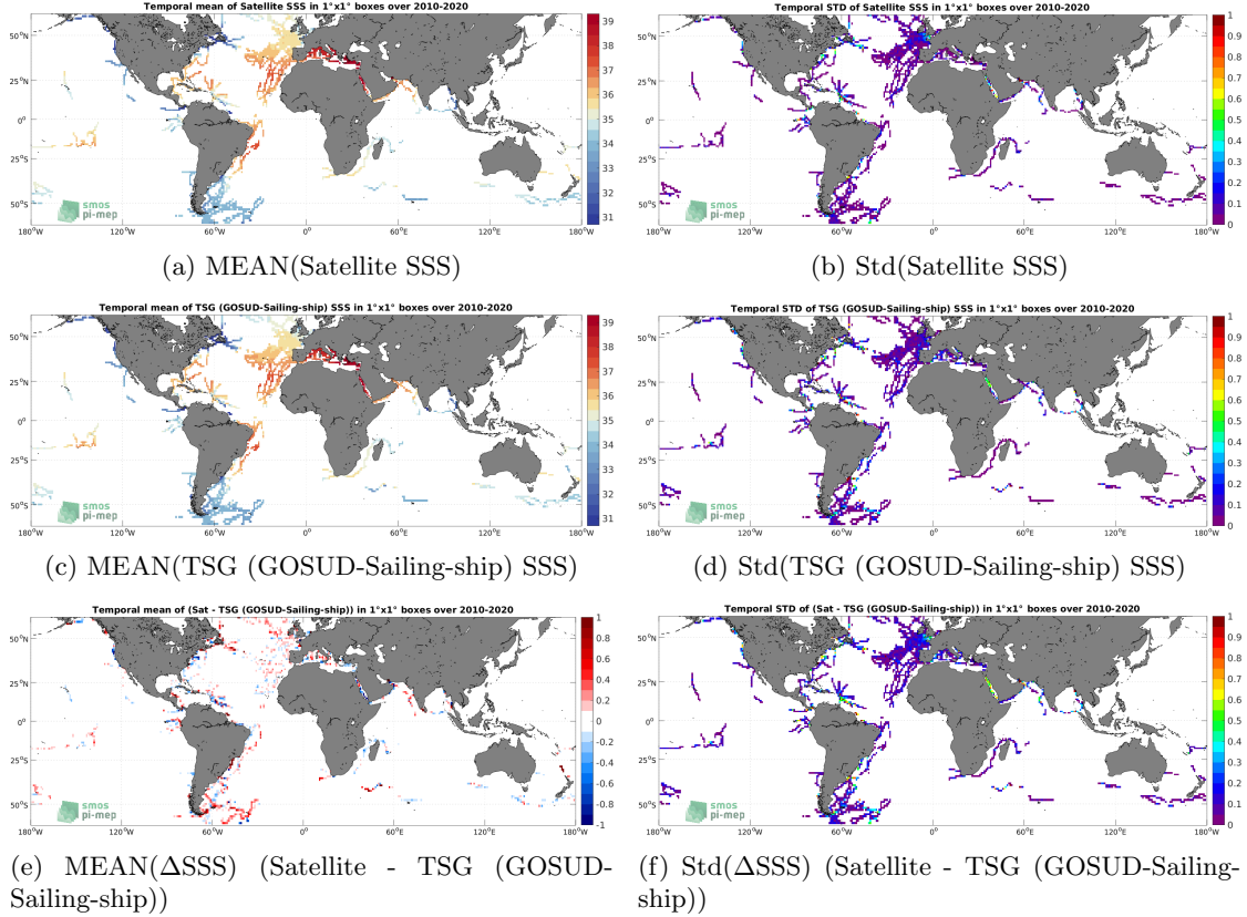
Figure 6: Temporal mean (left) and Std (right) of SSS from CCI SSS L4 Merged-OI v3.2 - 30-day running (ESA) (top), TSG (GOSUD-Sailing-ship) (middle), and of \Delta SSS (Satellite - TSG (GOSUD-Sailing-ship)). Only match-up pairs are used to generate these maps.
