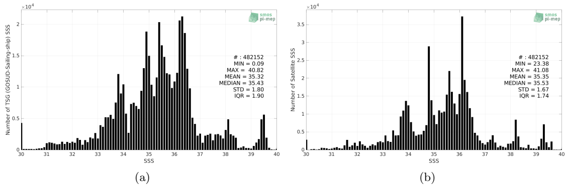
Figure 2: Histograms of SSS from TSG (GOSUD-Sailing-ship) (a) and CCI SSS L4 Merged-OI v3.2 - 30-day running (ESA) (b) considering all match-up pairs per bins of 0.1 over the SMOS coastal zone (<800km) 60N-60S Pi-MEP region and for the full satellite product period.
