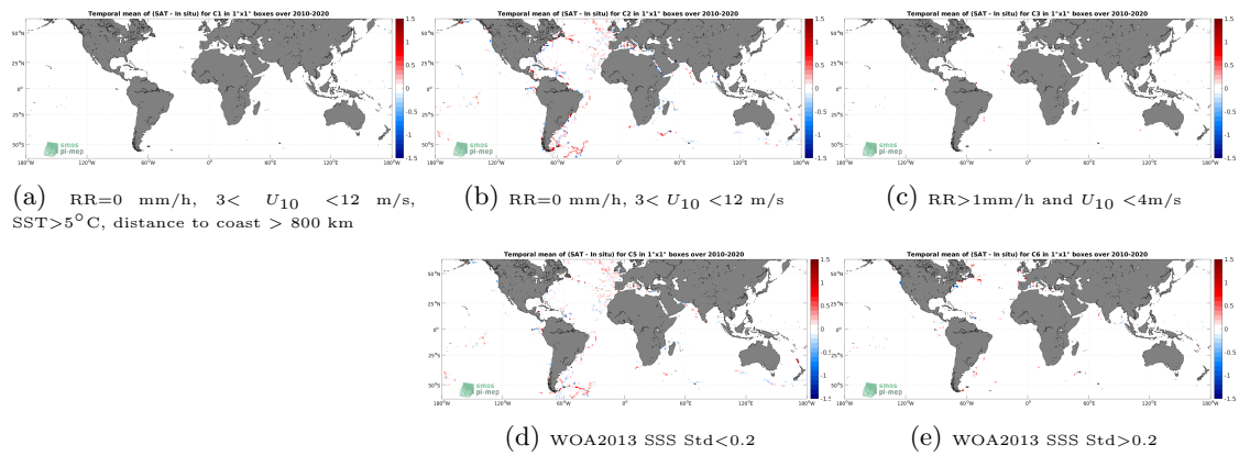
Figure 12: Temporal mean gridded over spatial boxes of size 1^\circ \times 1^\circ of \Delta SSS (CCI SSS L4 Merged-OI v3.2 - 30-day running (ESA) - TSG (GOSUD-Sailing-ship)) for 5 different subdatasets corresponding to:RR=0 mm/h, 3 < U_{10} < 12 m/s, SST >5^\circ\text{C} , distance to coast > 800 km (a), RR=0 mm/h, 3 < U_{10} < 12 m/s (b), RR >1 mm/h and U_{10} < 4 m/s (c), WOA2013 SSS Std <0.2 (d), WOA2013 SSS Std >0.2 (e).
