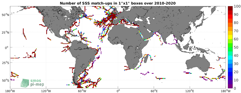
Figure 4: Number of SSS match-ups between TSG (GOSUD-Sailing-ship) SSS and the CCI SSS L4 Merged-OI v3.2 - 30-day running (ESA) SSS product for the SMOS coastal zone (<800km) 60N-60S Pi-MEP region over 1^\circ \times 1^\circ boxes and for the full satellite product period.
