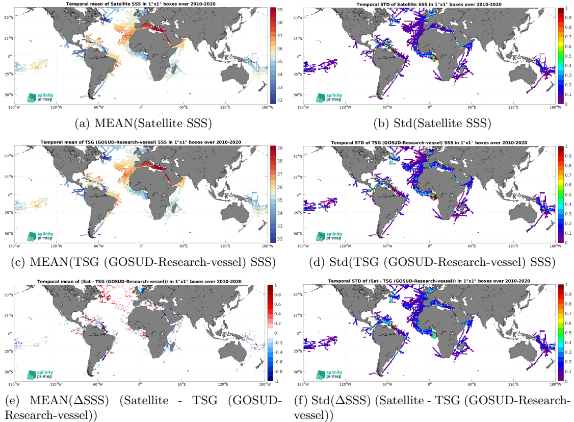
Figure 6: Temporal mean (left) and Std (right) of SSS from CCI SSS L4 Merged-OI v3.2 - 30-day running (ESA) (top), TSG (GOSUD-Research-vessel) (middle), and of \Delta\text{SSS} (Satellite - TSG (GOSUD-Research-vessel)). Only match-up pairs are used to generate these maps.
