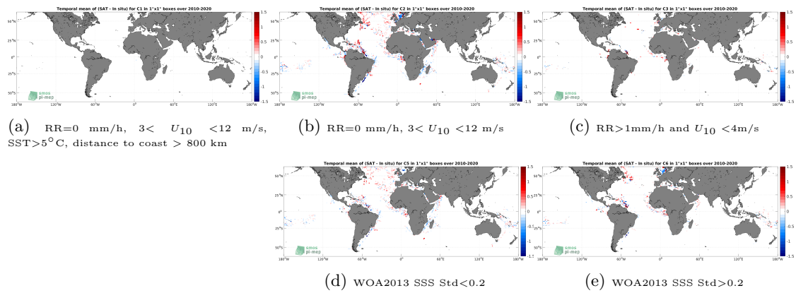
Figure 12: Temporal mean gridded over spatial boxes of size 1^\circ \times 1^\circ of \Delta SSS (CCI SSS L4 Merged-OI v3.2 - 30-day running (ESA) - TSG (GOSUD-Research-vessel)) for 5 different subdatasets corresponding to:RR=0 mm/h, 3 < U_{10} < 12 m/s, SST >5^\circ\text{C} , distance to coast > 800 km (a), RR=0 mm/h, 3 < U_{10} < 12 m/s (b), RR >1 mm/h and U_{10} < 4 m/s (c), WOA2013 SSS Std <0.2 (d), WOA2013 SSS Std >0.2 (e).
