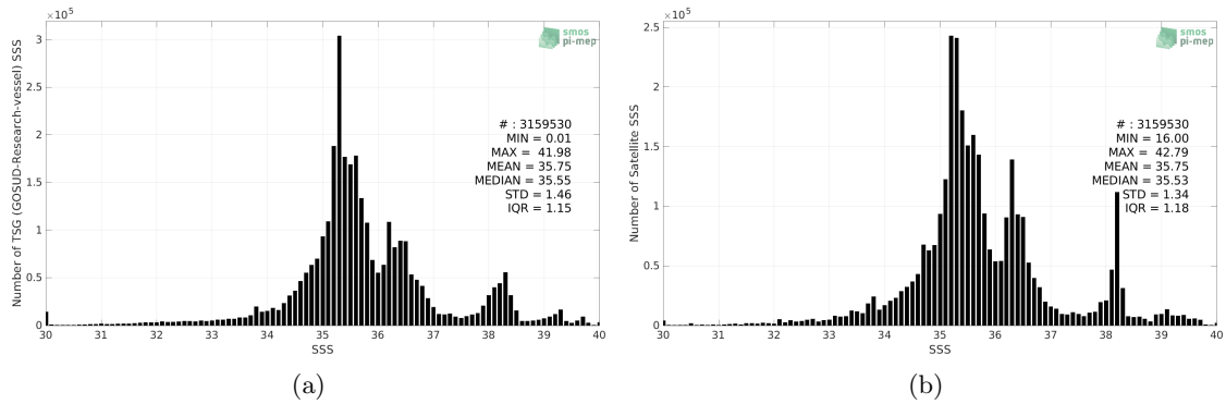
Figure 2: Histograms of SSS from TSG (GOSUD-Research-vessel) (a) and CCI SSS L4 Merged-OI v3.2 - 30-day running (ESA) (b) considering all match-up pairs per bins of 0.1 over the SMOS coastal zone (<800km) 60N-60S Pi-MEP region and for the full satellite product period.
