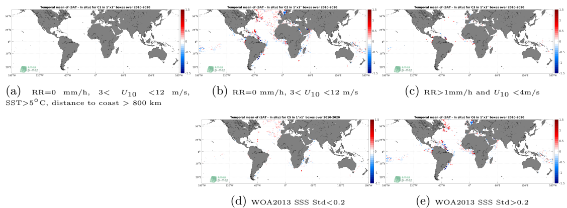
Figure 12: Temporal mean gridded over spatial boxes of size 1^\circ \times 1^\circ of \Delta\text{SSS} (CCI SSS L4 Merged-OI v3.2 - 30-day running (ESA) - TSG (GOSUD-Research-vessel)) for 5 different subdatasets corresponding to:RR=0 mm/h, 3 < U_{10} < 12 m/s, SST >5^\circ\text{C} , distance to coast > 800 km (a), RR=0 mm/h, 3 < U_{10} < 12 m/s (b), RR >1 mm/h and U_{10} < 4 m/s (c), WOA2013 SSS Std <0.2 (d), WOA2013 SSS Std >0.2 (e).
