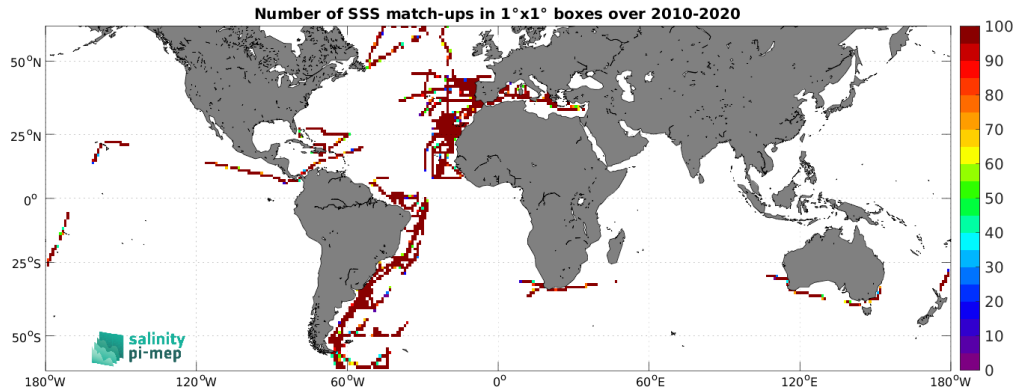
Figure 4: Number of SSS match-ups between TSG (CSIC-UTM) SSS and the CCI SSS L4 Merged-OI v3.2 - 30-day running (ESA) SSS product for the SMOS coastal zone ( <800\text{km} ) 60N-60S Pi-MEP region over 1^\circ \times 1^\circ boxes and for the full satellite product period.
