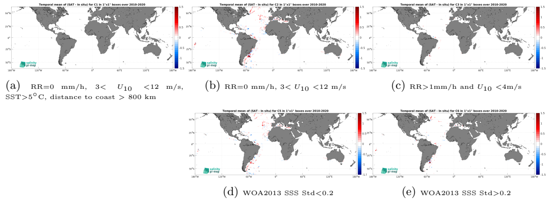
Figure 12: Temporal mean gridded over spatial boxes of size 1^\circ \times 1^\circ of \Delta SSS (CCI SSS L4 Merged-OI v3.2 - 30-day running (ESA) - TSG (CSIC-UTM)) for 5 different subdatasets corresponding to:RR=0 mm/h, 3 < U_{10} < 12 m/s, SST >5^\circ C, distance to coast > 800 km (a), RR=0 mm/h, 3 < U_{10} < 12 m/s (b), RR >1 mm/h and U_{10} < 4 m/s (c), WOA2013 SSS Std <0.2 (d), WOA2013 SSS Std >0.2 (e).
