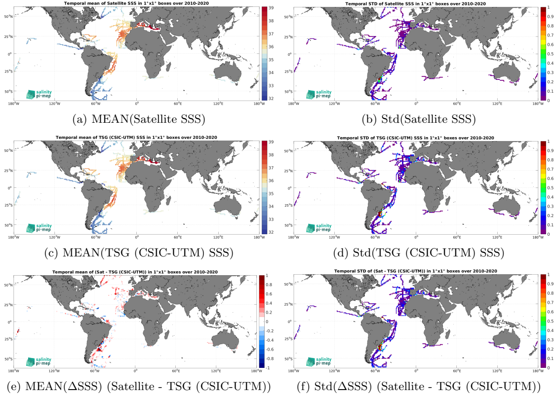
Figure 6: Temporal mean (left) and Std (right) of SSS from CCI SSS L4 Merged-OI v3.2 - 30-day running (ESA) (top), TSG (CSIC-UTM) (middle), and of \Delta\text{SSS} (Satellite - TSG (CSIC-UTM)). Only match-up pairs are used to generate these maps.
