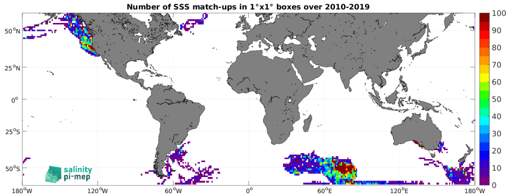
Figure 4: Number of SSS match-ups between Marine mammals SSS and the CCI SSS L4 Merged-OI v3.2 - 30-day running (ESA) SSS product for the SMOS coastal zone (<800km) 60N-60S Pi-MEP region over 1^\circ \times 1^\circ boxes and for the full satellite product period.
