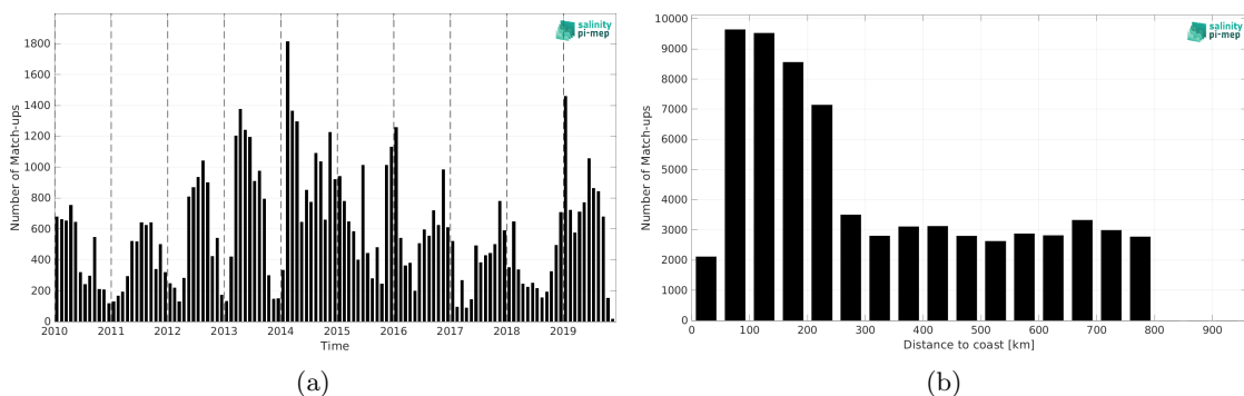
Figure 1: Number of match-ups between Marine mammals and CCI SSS L4 Merged-OI v3.2 - 30-day running (ESA) SSS as a function of time (a) and as function of the distance to coast (b) over the SMOS coastal zone (<800km) 60N-60S Pi-MEP region and for the full satellite product period.
