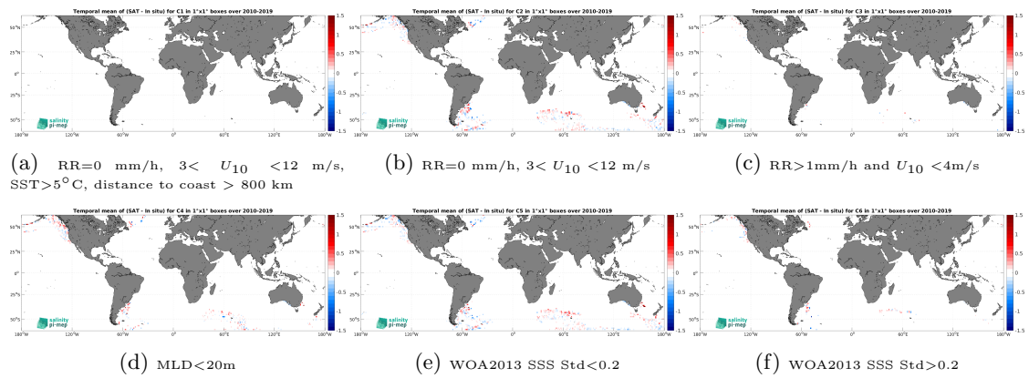
Figure 12: Temporal mean gridded over spatial boxes of size 1^\circ \times 1^\circ of \Delta SSS (CCI SSS L4 Merged-OI v3.2 - 30-day running (ESA) - Marine mammals) for 6 different subdatasets corresponding to:RR=0 mm/h, 3 < U_{10} < 12 m/s, SST >5^\circ C, distance to coast > 800 km (a), RR=0 mm/h, 3 < U_{10} < 12 m/s (b), RR >1 mm/h and U_{10} < 4 m/s (c),MLD <20 m (d),WOA2013 SSS Std <0.2 (e),WOA2013 SSS Std >0.2 (f).
