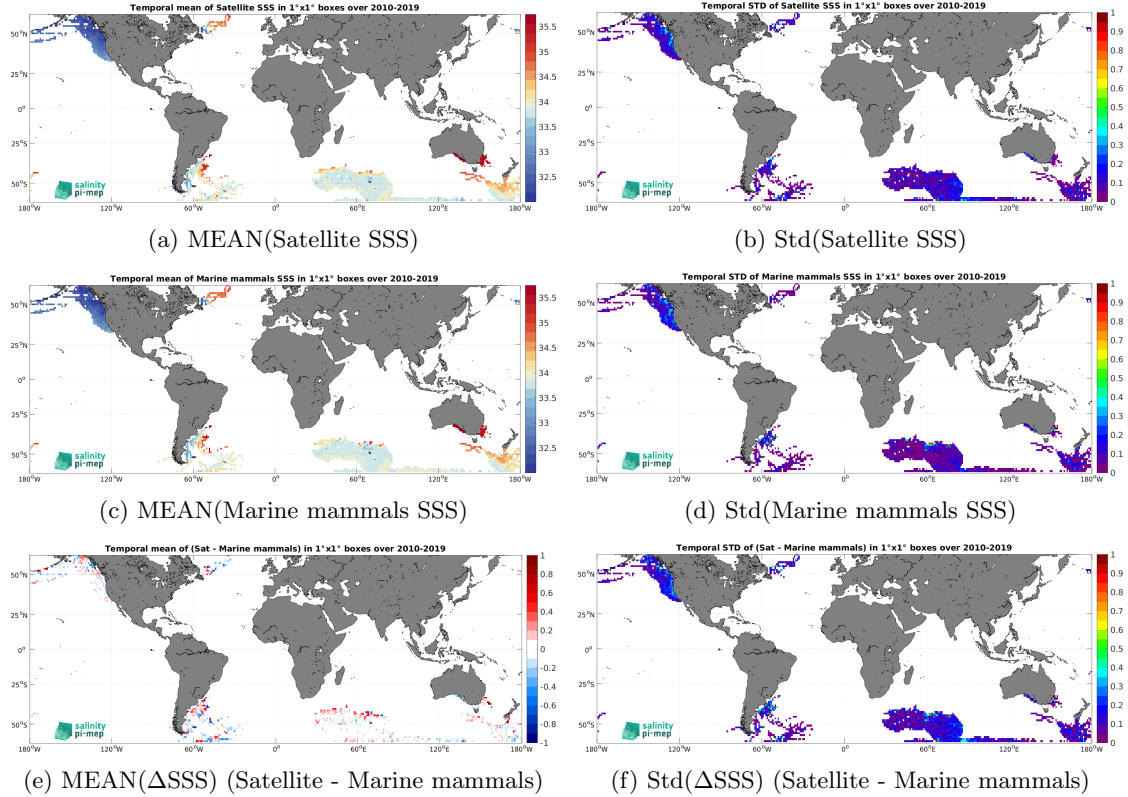
Figure 6: Temporal mean (left) and Std (right) of SSS from CCI SSS L4 Merged-OI v3.2 - 30-day running (ESA) (top), Marine mammals (middle), and of \Delta SSS (Satellite - Marine mammals). Only match-up pairs are used to generate these maps.
