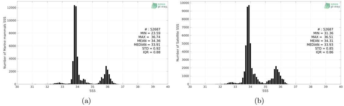
Figure 2: Histograms of SSS from Marine mammals (a) and CCI SSS L4 Merged-OI v3.2 - 30-day running (ESA) (b) considering all match-up pairs per bins of 0.1 over the SMOS coastal zone (<800km) 60N-60S Pi-MEP region and for the full satellite product period.
