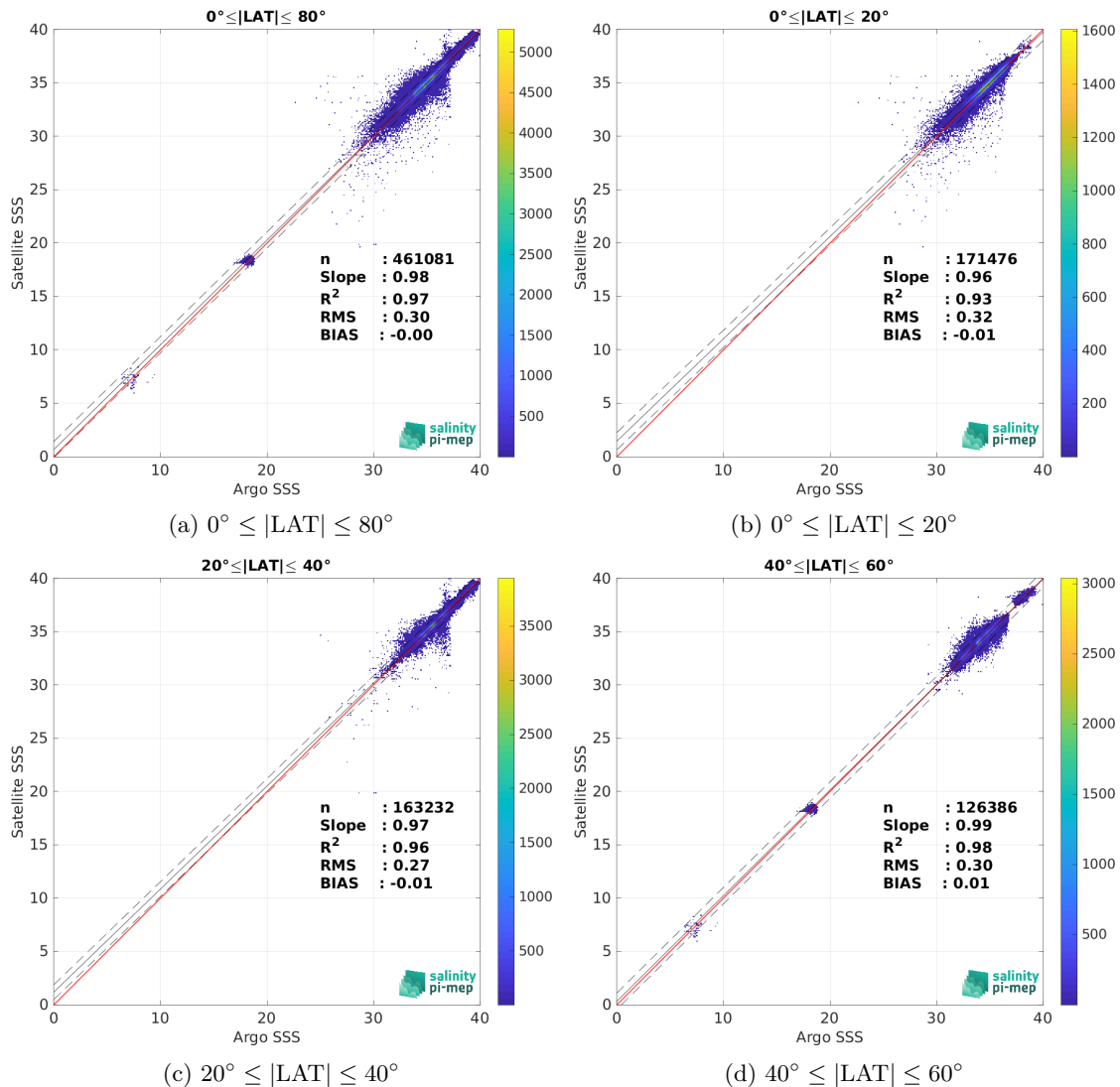
Figure 9: Contour maps of the concentration of CCI SSS L4 Merged-OI v3.2 - 30-day running (ESA) SSS (y-axis) versus Argo SSS (x-axis) at match-up pairs for different latitude bands. For each plot, the red line shows x=y . The black thin and dashed lines indicate a linear fit through the data cloud and the \pm 95\% confidence levels, respectively. The number match-up pairs n , the slope and R^2 coefficient of the linear fit, the root mean square (RMS) and the mean bias between satellite and in situ data are indicated for each latitude band in each plots.
