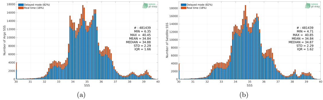
Figure 2: Histograms of SSS from Argo (a) and CCI SSS L4 Merged-OI v3.2 - 30-day running (ESA) (b) considering all match-up pairs per bins of 0.1 over the SMOS coastal zone (<800km) 60N-60S Pi-MEP region and for the full satellite product period.
