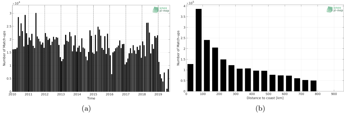
Figure 1: Number of match-ups between TSG (LEGOS-DM) and CCI L4 Merged-OI v2.31 - 30-day running (ESA) SSS as a function of time (a) and as function of the distance to coast (b) over the SMOS coastal zone (<800km) 60N-60S Pi-MEP region and for the full satellite product period.
