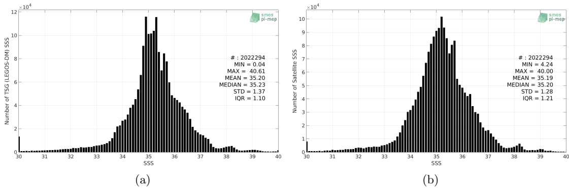
Figure 2: Histograms of SSS from TSG (LEGOS-DM) (a) and CCI L4 Merged-OI v2.31 - 30-day running (ESA) (b) considering all match-up pairs per bins of 0.1 over the SMOS coastal zone (<800km) 60N-60S Pi-MEP region and for the full satellite product period.
