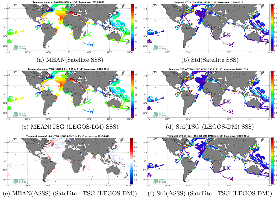
Figure 6: Temporal mean (left) and Std (right) of SSS from CCI L4 Merged-OI v2.31 - 30-day running (ESA) (top), TSG (LEGOS-DM) (middle), and of \Delta SSS (Satellite - TSG (LEGOS-DM)). Only match-up pairs are used to generate these maps.
