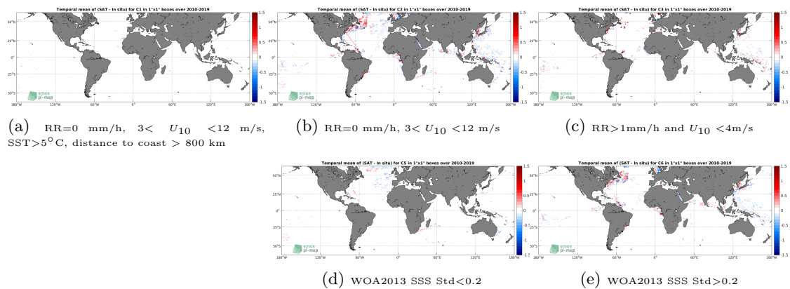
Figure 12: Temporal mean gridded over spatial boxes of size 1^\circ \times 1^\circ of \Delta SSS (CCI L4 Merged-OI v2.31 - 30-day running (ESA) - TSG (LEGOS-DM)) for 5 different subdatasets corresponding to:RR=0 mm/h, 3 < U_{10} < 12 m/s, SST >5^\circ C, distance to coast > 800 km (a), RR=0 mm/h, 3 < U_{10} < 12 m/s (b), RR >1 mm/h and U_{10} < 4 m/s (c), WOA2013 SSS Std <0.2 (d), WOA2013 SSS Std >0.2 (e).
