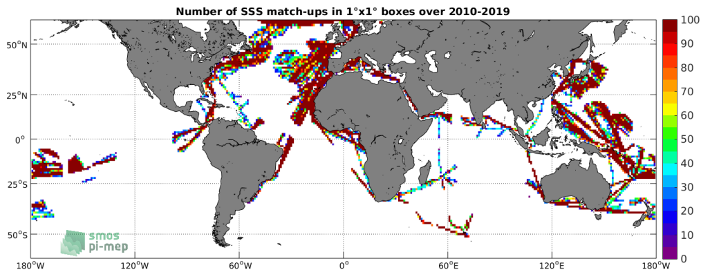
Figure 4: Number of SSS match-ups between TSG (LEGOS-DM) SSS and the CCI L4 Merged-OI v2.31 - 30-day running (ESA) SSS product for the SMOS coastal zone (<800km) 60N-60S Pi-MEP region over 1°x1° boxes and for the full satellite product period.
