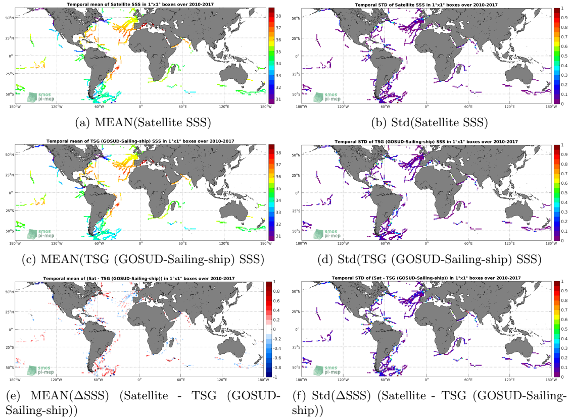
Figure 6: Temporal mean (left) and Std (right) of SSS from CCI SSS L4 Merged-OI v2.31 - 30-day running (ESA) (top), TSG (GOSUD-Sailing-ship) (middle), and of \Delta SSS (Satellite - TSG (GOSUD-Sailing-ship)). Only match-up pairs are used to generate these maps.
