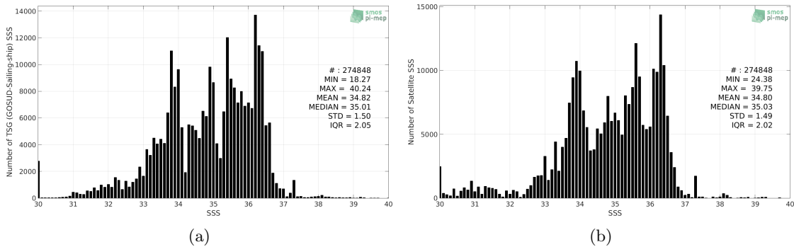
Figure 2: Histograms of SSS from TSG (GOSUD-Sailing-ship) (a) and CCI SSS L4 Merged-OI v2.31 - 30-day running (ESA) (b) considering all match-up pairs per bins of 0.1 over the SMOS coastal zone (<800km) 60N-60S Pi-MEP region and for the full satellite product period.
