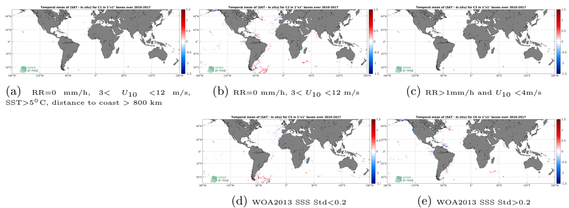
Figure 12: Temporal mean gridded over spatial boxes of size 1^\circ \times 1^\circ of \Delta\text{SSS} (CCI SSS L4 Merged-OI v2.31 - 30-day running (ESA) - TSG (GOSUD-Sailing-ship)) for 5 different subdatasets corresponding to: RR=0 mm/h, 3 < U_{10} < 12 m/s, SST > 5°C, distance to coast > 800 km (a), RR=0 mm/h, 3 < U_{10} < 12 m/s (b), RR > 1mm/h and U_{10} < 4 m/s (c), WOA2013 SSS Std < 0.2 (d), WOA2013 SSS Std > 0.2 (e).
