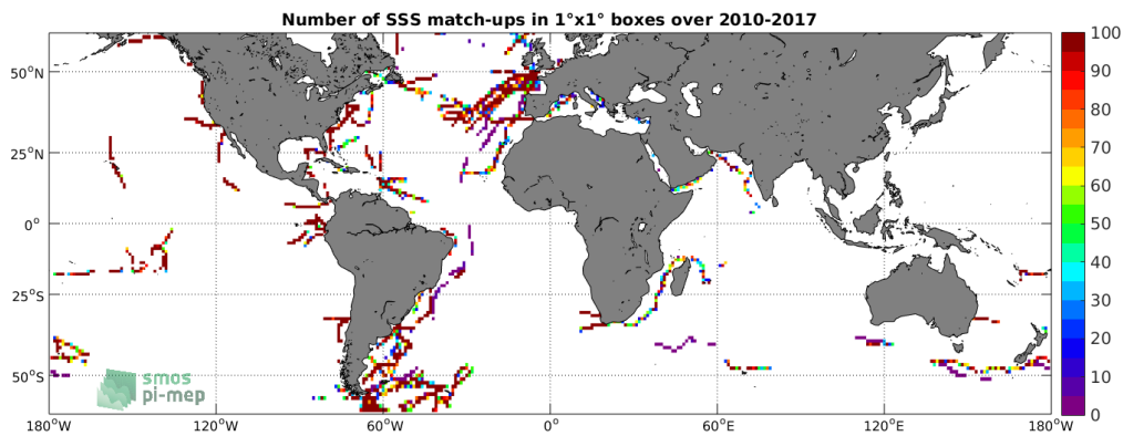
Figure 4: Number of SSS match-ups between TSG (GOSUD-Sailing-ship) SSS and the CCI SSS L4 Merged-OI v2.31 - 30-day running (ESA) SSS product for the SMOS coastal zone (<800km) 60N-60S Pi-MEP region over 1^\circ \times 1^\circ boxes and for the full satellite product period.
