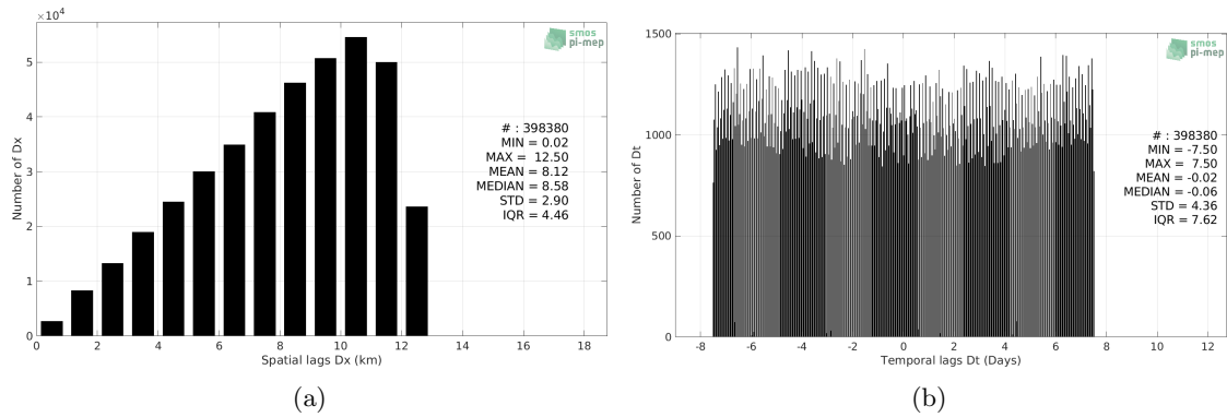
Figure 4: Histograms of the spatial (a) and temporal (b) lags between the location/time of the Surface drifters measurement and the date of the corresponding CCI SSS L4 Merged-OI v2.31 - 30-day running (ESA) SSS pixel.
