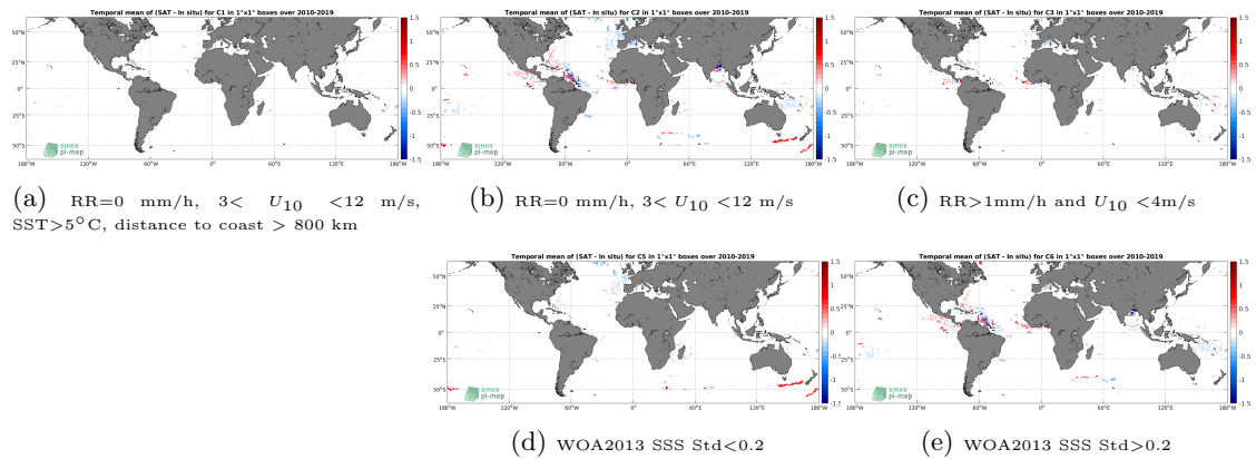
Figure 11: Temporal mean gridded over spatial boxes of size 1^\circ \times 1^\circ of \Delta\text{SSS} (CCI SSS L4 Merged-OI v2.31 - 30-day running (ESA) - Surface drifters) for 5 different subdatasets corresponding to:RR=0 mm/h, 3 < U_{10} < 12 m/s, SST >5^\circ\text{C} , distance to coast > 800 km (a), RR=0 mm/h, 3 < U_{10} < 12 m/s (b), RR >1 mm/h and U_{10} < 4 m/s (c), WOA2013 SSS Std <0.2 (d), WOA2013 SSS Std >0.2 (e).
