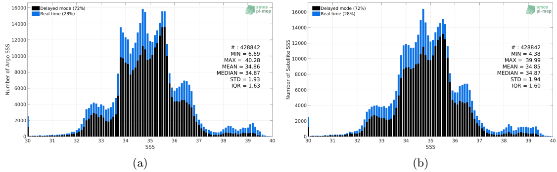
Figure 2: Histograms of SSS from Argo (a) and CCI L4 Merged-OI v2.31 - 30-day running (ESA) (b) considering all match-up pairs per bins of 0.1 over the SMOS coastal zone (<800km) 60N-60S Pi-MEP region and for the full satellite product period.
