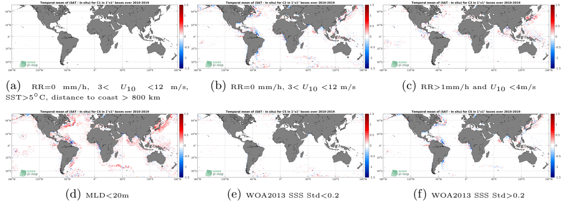
Figure 12: Temporal mean gridded over spatial boxes of size 1^\circ \times 1^\circ of \Delta SSS (CCI L4 Merged-OI v2.31 - 30-day running (ESA) - Argo) for 6 different subdatasets corresponding to: RR=0 mm/h, 3 < U_{10} < 12 m/s, SST > 5^\circ C , distance to coast > 800 km (a), RR=0 mm/h, 3 < U_{10} < 12 m/s (b), RR > 1 mm/h and U_{10} < 4 m/s (c), MLD < 20 m (d), WOA2013 SSS Std < 0.2 (e), WOA2013 SSS Std > 0.2 (f).
