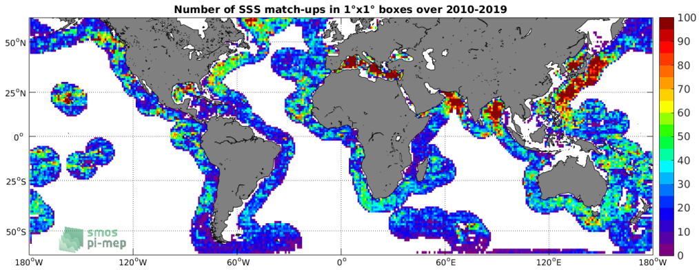
Figure 4: Number of SSS match-ups between Argo SSS and the CCI L4 Merged-OI v2.31 - 30-day running (ESA) SSS product for the SMOS coastal zone (<800km) 60N-60S Pi-MEP region over 1°x1° boxes and for the full satellite product period.
