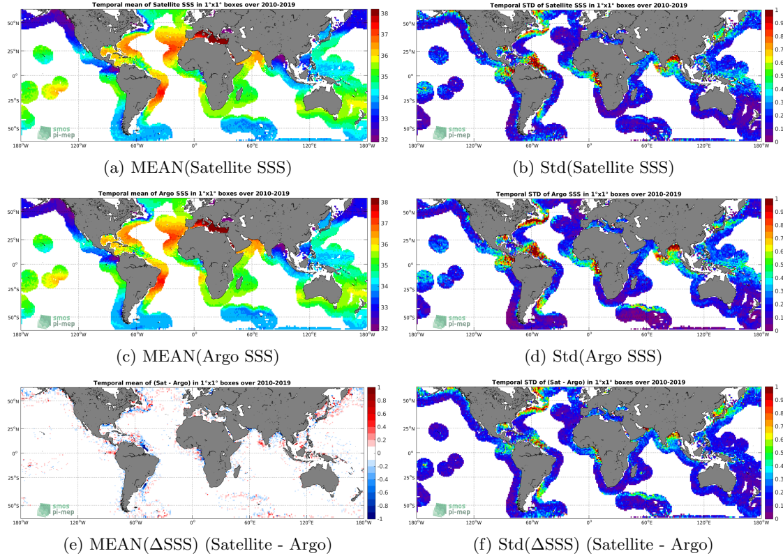
Figure 6: Temporal mean (left) and Std (right) of SSS from CCI L4 Merged-OI v2.31 - 30-day running (ESA) (top), Argo (middle), and of \Delta SSS (Satellite - Argo). Only match-up pairs are used to generate these maps.
