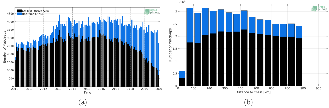
Figure 1: Number of match-ups between Argo and CCI L4 Merged-OI v2.31 - 30-day running (ESA) SSS as a function of time (a) and as function of the distance to coast (b) over the SMOS coastal zone (<800km) 60N-60S Pi-MEP region and for the full satellite product period.
