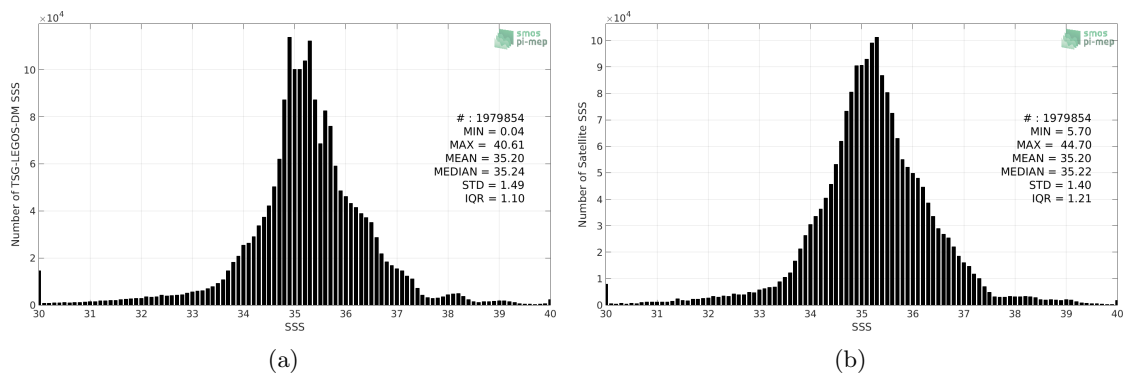
Figure 2: Histograms of SSS from TSG-LEGOS-DM (a) and CCI L4 Merged-OI v1.8 - 7-day running (ESA) (b) considering all match-up pairs per bins of 0.1 over the SMOS coastal zone (<800km) 60N-60S Pi-MEP region and for the full satellite product period.
