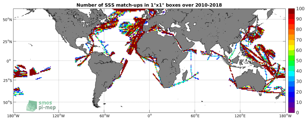
Figure 4: Number of SSS match-ups between TSG-LEGOS-DM SSS and the CCI L4 Merged-OI v1.8 - 7-day running (ESA) SSS product for the SMOS coastal zone (<800km) 60N-60S Pi-MEP region over 1^\circ \times 1^\circ boxes and for the full satellite product period.
