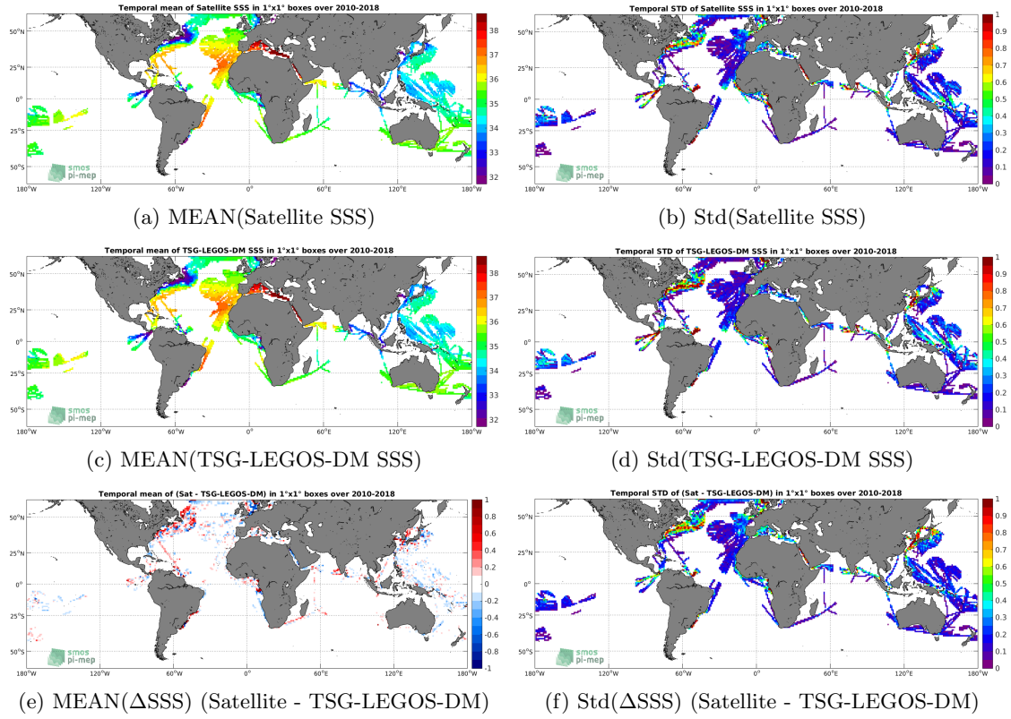
Figure 6: Temporal mean (left) and Std (right) of SSS from CCI L4 Merged-OI v1.8 - 7-day running (ESA) (top), TSG-LEGOS-DM (middle), and of \Delta SSS (Satellite - TSG-LEGOS-DM). Only match-up pairs are used to generate these maps.
