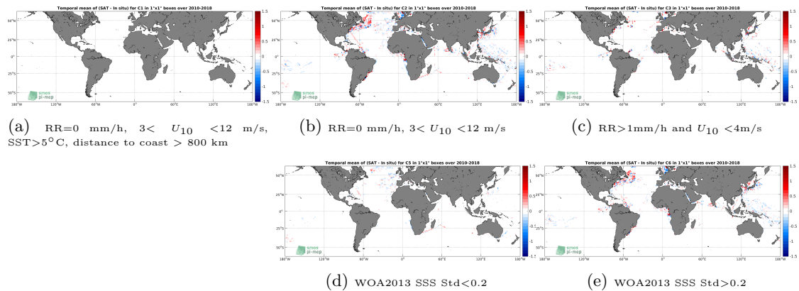
Figure 12: Temporal mean gridded over spatial boxes of size 1^\circ \times 1^\circ of \Delta SSS (CCI L4 Merged-OI v1.8 - 7-day running (ESA) - TSG-LEGOS-DM) for 5 different subdatasets corresponding to:RR=0 mm/h, 3 < U_{10} < 12 m/s, SST >5^\circ C, distance to coast > 800 km (a), RR=0 mm/h, 3 < U_{10} < 12 m/s (b), RR >1 mm/h and U_{10} < 4 m/s (c), WOA2013 SSS Std <0.2 (d), WOA2013 SSS Std >0.2 (e).
