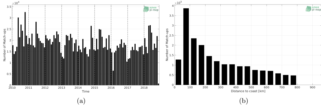
Figure 1: Number of match-ups between TSG-LEGOS-DM and CCI L4 Merged-OI v1.8 - 7-day running (ESA) SSS as a function of time (a) and as function of the distance to coast (b) over the SMOS coastal zone (<800km) 60N-60S Pi-MEP region and for the full satellite product period.
