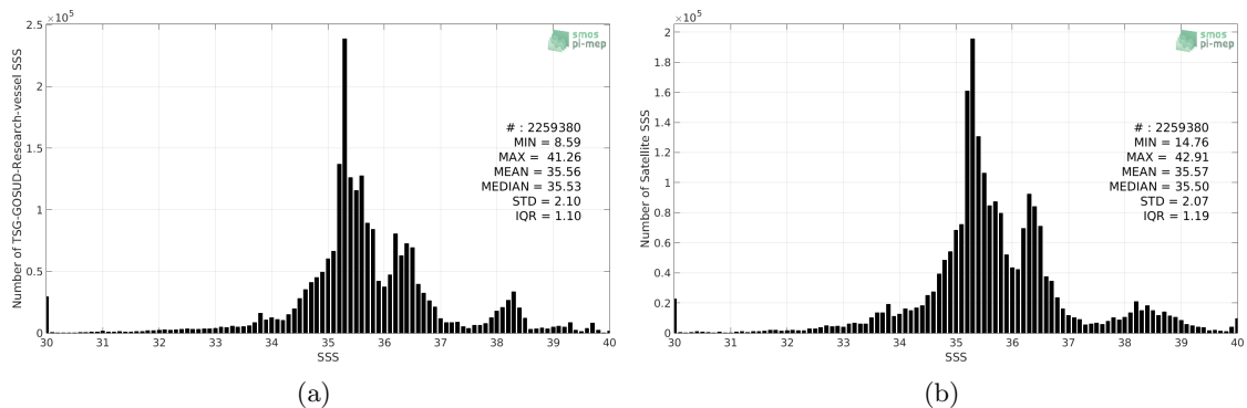
Figure 2: Histograms of SSS from TSG-GOSUD-Research-vessel (a) and CCI L4 Merged-OI v1.8 - 7-day running (ESA) (b) considering all match-up pairs per bins of 0.1 over the SMOS coastal zone (<800km) 60N-60S Pi-MEP region and for the full satellite product period.
