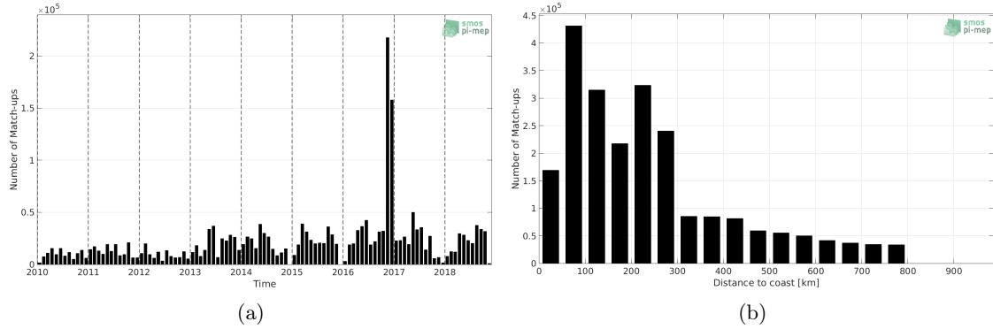
Figure 1: Number of match-ups between TSG-GOSUD-Research-vessel and CCI L4 Merged-OI v1.8 - 7-day running (ESA) SSS as a function of time (a) and as function of the distance to coast (b) over the SMOS coastal zone (<800km) 60N-60S Pi-MEP region and for the full satellite product period.
