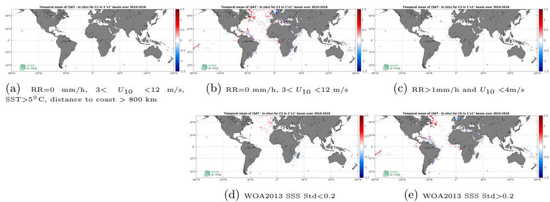
Figure 12: Temporal mean gridded over spatial boxes of size 1^\circ \times 1^\circ of \Delta SSS (CCI L4 Merged-OI v1.8 - 7-day running (ESA) - TSG-GOSUD-Research-vessel) for 5 different subdatasets corresponding to: RR=0 mm/h, 3 < U_{10} < 12 m/s, SST > 5^\circ\text{C} , distance to coast > 800 km (a), RR=0 mm/h, 3 < U_{10} < 12 m/s (b), RR > 1 mm/h and U_{10} < 4 m/s (c), WOA2013 SSS Std < 0.2 (d), WOA2013 SSS Std > 0.2 (e).
