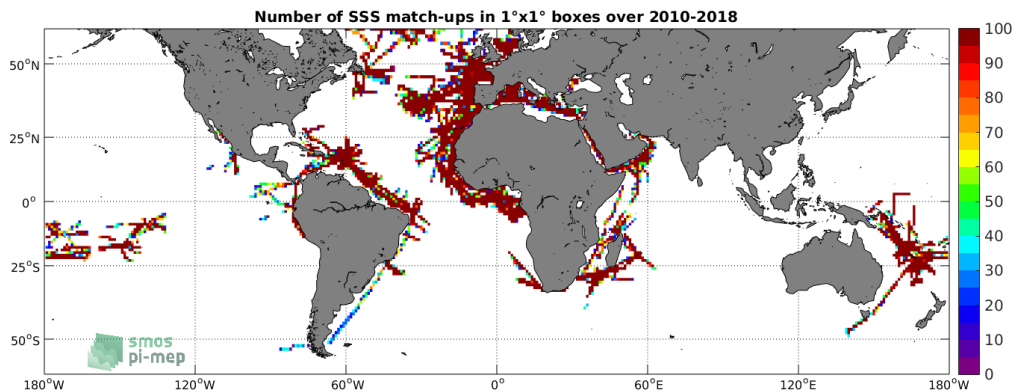
Figure 4: Number of SSS match-ups between TSG-GOSUD-Research-vessel SSS and the CCI L4 Merged-OI v1.8 - 7-day running (ESA) SSS product for the SMOS coastal zone (<800km) 60N-60S Pi-MEP region over 1^\circ \times 1^\circ boxes and for the full satellite product period.
