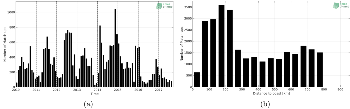
Figure 1: Number of match-ups between Sea mammals and CCI-L4-ESA-MERGED-OI-V1.8-7DAY-RUNNING SSS as a function of time (a) and as function of the distance to coast (b) over the SMOS coastal zone ( \approx 800\text{km} ) 60N-60S Pi-MEP region and for the full satellite product period.
