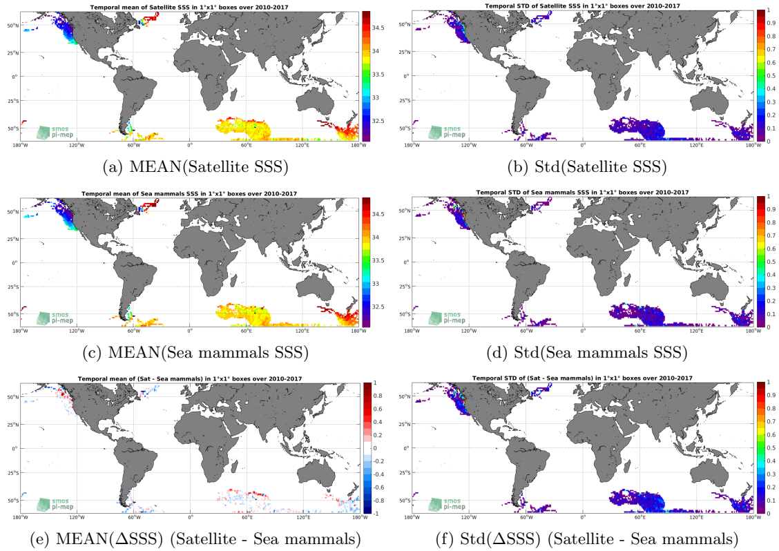
Figure 6: Temporal mean (left) and Std (right) of SSS from CCI-L4-ESA-MERGED-OI-V1.8-7DAY-RUNNING (top), Sea mammals (middle), and of \Delta SSS (Satellite - Sea mammals). Only match-up pairs are used to generate these maps.
