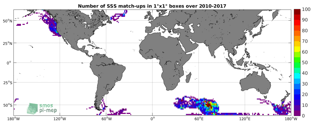
Figure 4: Number of SSS match-ups between Sea mammals SSS and the CCI-L4-ESA-MERGED-OI-V1.8-7DAY-RUNNING SSS product for the SMOS coastal zone ( \pm 800\text{km} ) 60N-60S Pi-MEP region over 1^\circ \times 1^\circ boxes and for the full satellite product period.
