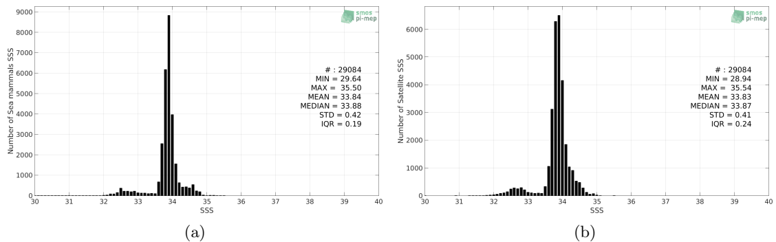
Figure 2: Histograms of SSS from Sea mammals (a) and CCI-L4-ESA-MERGED-OI-V1.8-7DAY-RUNNING (b) considering all match-up pairs per bins of 0.1 over the SMOS coastal zone ( \approx 800\text{km} ) 60N-60S Pi-MEP region and for the full satellite product period.
