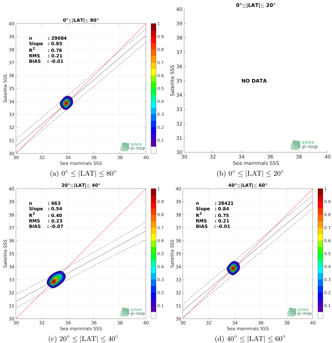
Figure 9: Contour maps of the concentration of CCI-L4-ESA-MERGED-OI-V1.8-7DAY-RUNNING SSS (y-axis) versus Sea mammals SSS (x-axis) at match-up pairs for different latitude bands. For each plot, the red line shows x=y . The black thin and dashed lines indicate a linear fit through the data cloud and the \pm 95\% confidence levels, respectively. The number match-up pairs n , the slope and R^2 coefficient of the linear fit, the root mean square (RMS) and the mean bias between satellite and in situ data are indicated for each latitude band in each plots.
