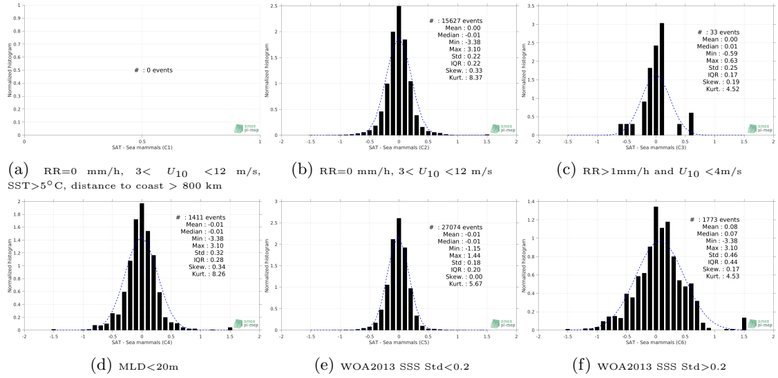
Figure 13: Normalized histogram of \Delta SSS (CCI-L4-ESA-MERGED-OI-V1.8-7DAY-RUNNING - Sea mammals) for 6 different subdatasets corresponding to: RR=0 mm/h, 3 < U_{10} < 12 m/s, SST>5°C, distance to coast > 800 km (a), RR=0 mm/h, 3 < U_{10} < 12 m/s (b), RR>1mm/h and U_{10} < 4 m/s (c), MLD<20m (d), WOA2013 SSS Std<0.2 (e), WOA2013 SSS Std>0.2 (f).
