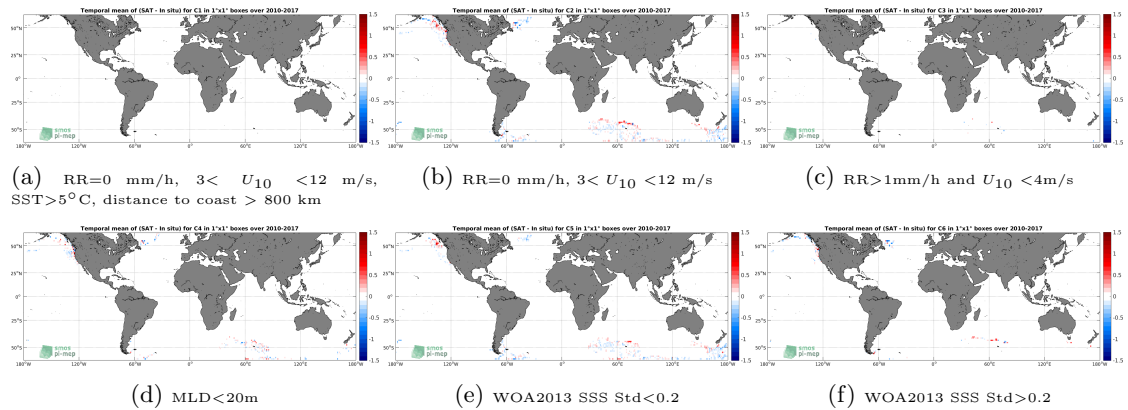
Figure 12: Temporal mean gridded over spatial boxes of size 1^\circ \times 1^\circ of \Delta SSS (CCI-L4-ESA-MERGED-OI-V1.8-7DAY-RUNNING - Sea mammals) for 6 different subdatasets corresponding to:RR=0 mm/h, 3 < U_{10} < 12 m/s, SST >5^\circ C, distance to coast > 800 km (a), RR=0 mm/h, 3 < U_{10} < 12 m/s (b), RR >1 mm/h and U_{10} < 4 m/s (c),MLD <20 m (d),WOA2013 SSS Std <0.2 (e),WOA2013 SSS Std >0.2 (f).
