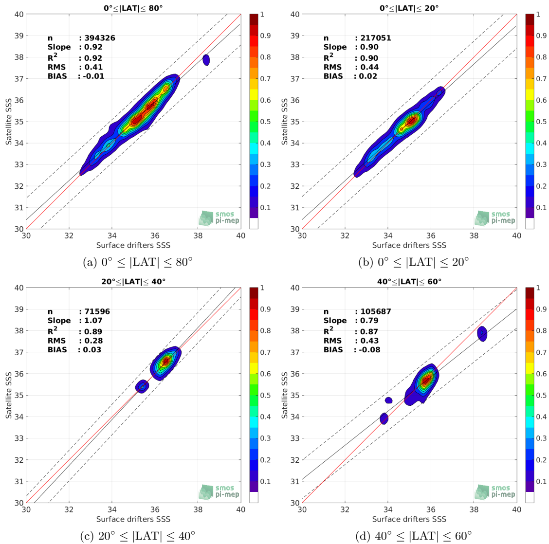
Figure 8: Contour maps of the concentration of CCI L4 Merged-OI v1.8 - 7-day running (ESA) SSS (y-axis) versus Surface drifters SSS (x-axis) at match-up pairs for different latitude bands. For each plot, the red line shows x=y . The black thin and dashed lines indicate a linear fit through the data cloud and the \pm 95\% confidence levels, respectively. The number match-up pairs n , the slope and R^2 coefficient of the linear fit, the root mean square (RMS) and the mean bias between satellite and in situ data are indicated for each latitude band in each plots.
