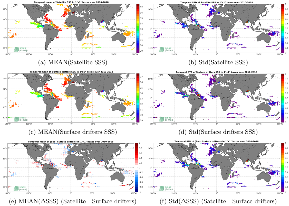
Figure 5: Temporal mean (left) and Std (right) of SSS from CCI L4 Merged-OI v1.8 - 7-day running (ESA) (top), Surface drifters (middle), and of \Delta SSS (Satellite - Surface drifters). Only match-up pairs are used to generate these maps.
