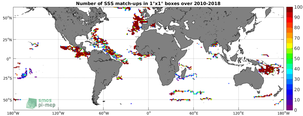
Figure 3: Number of SSS match-ups between Surface drifters SSS and the CCI L4 Merged-OI v1.8 - 7-day running (ESA) SSS product for the SMOS coastal zone (<800km) 60N-60S Pi-MEP region over 1°x1° boxes and for the full satellite product period.
