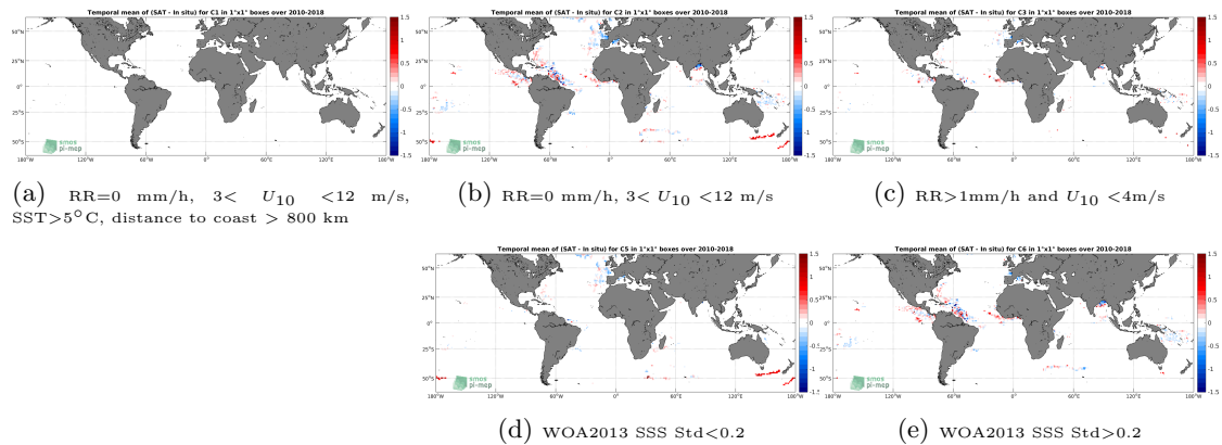
Figure 11: Temporal mean gridded over spatial boxes of size 1^\circ \times 1^\circ of \Delta SSS (CCI L4 Merged-OI v1.8 - 7-day running (ESA) - Surface drifters) for 5 different subdatasets corresponding to:RR=0 mm/h, 3 < U_{10} < 12 m/s, SST >5^\circ\text{C} , distance to coast > 800 km (a), RR=0 mm/h, 3 < U_{10} < 12 m/s (b), RR >1 mm/h and U_{10} < 4 m/s (c), WOA2013 SSS Std <0.2 (d), WOA2013 SSS Std >0.2 (e).
