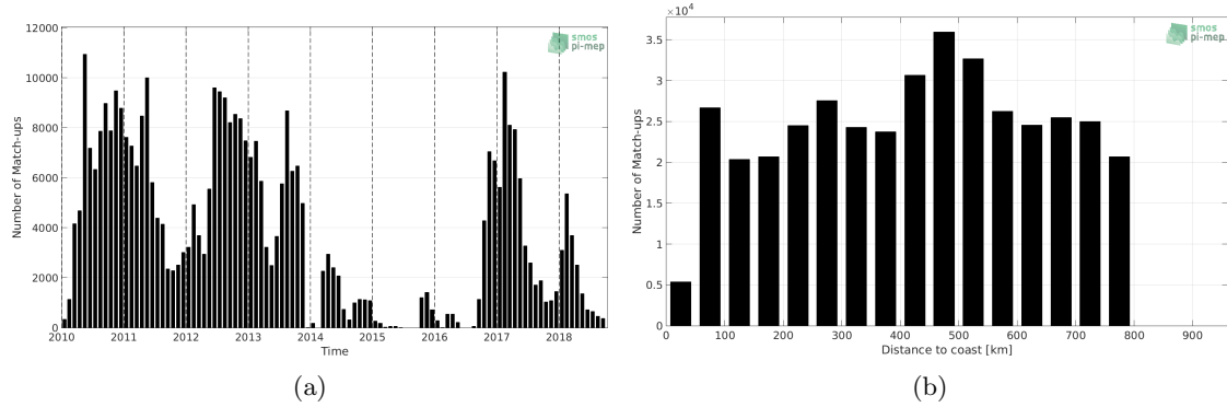
Figure 1: Number of match-ups between Surface drifters and CCI L4 Merged-OI v1.8 - 7-day running (ESA) SSS as a function of time (a) and as function of the distance to coast (b) over the SMOS coastal zone (<800km) 60N-60S Pi-MEP region and for the full satellite product period.
