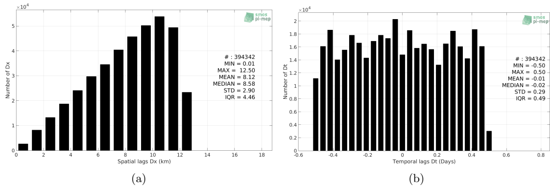
Figure 4: Histograms of the spatial (a) and temporal (b) lags between the time of the Surface drifters measurements and the date of the corresponding CCI L4 Merged-OI v1.8 - 7-day running (ESA) SSS product.
