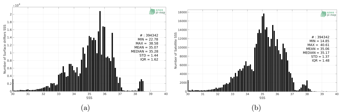
Figure 2: Histograms of SSS from Surface drifters (a) and CCI L4 Merged-OI v1.8 - 7-day running (ESA) (b) considering all match-up pairs per bins of 0.1 over the SMOS coastal zone (<800km) 60N-60S Pi-MEP region and for the full satellite product period.
