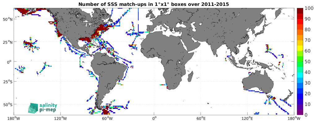
Figure 5: Number of SSS match-ups between TSG (SAMOS) SSS and the Aquarius SSS L4 OI v5 - Weekly (IPRC) SSS product for the SMOS coastal zone (<800km) 60N-60S Pi-MEP region over 1^{\circ} \times 1^{\circ} boxes and for the full satellite product period.
