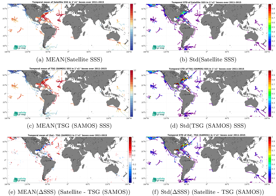
Figure 7: Temporal mean (left) and Std (right) of SSS from Aquarius SSS L4 OI v5 - Weekly (IPRC) (top), TSG (SAMOS) (middle), and of \Delta SSS (Satellite - TSG (SAMOS)). Only match-up pairs are used to generate these maps.
