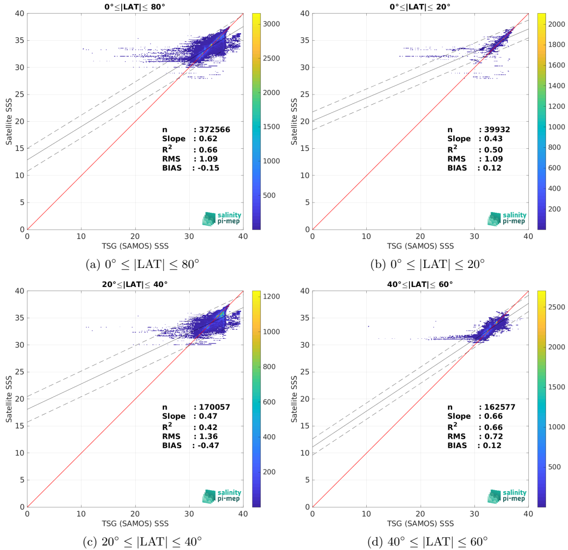
Figure 10: Contour maps of the concentration of Aquarius SSS L4 OI v5 - Weekly (IPRC) SSS (y-axis) versus TSG (SAMOS) SSS (x-axis) at match-up pairs for different latitude bands. For each plot, the red line shows x=y . The black thin and dashed lines indicate a linear fit through the data cloud and the \pm 95\% confidence levels, respectively. The number match-up pairs n , the slope and R^2 coefficient of the linear fit, the root mean square (RMS) and the mean bias between satellite and in situ data are indicated for each latitude band in each plots.
