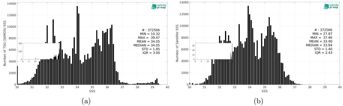
Figure 3: Histograms of SSS from TSG (SAMOS) (a) and Aquarius SSS L4 OI v5 - Weekly (IPRC) (b) considering all match-up pairs per bins of 0.1 over the SMOS coastal zone (<800km) 60N-60S Pi-MEP region and for the full satellite product period.
