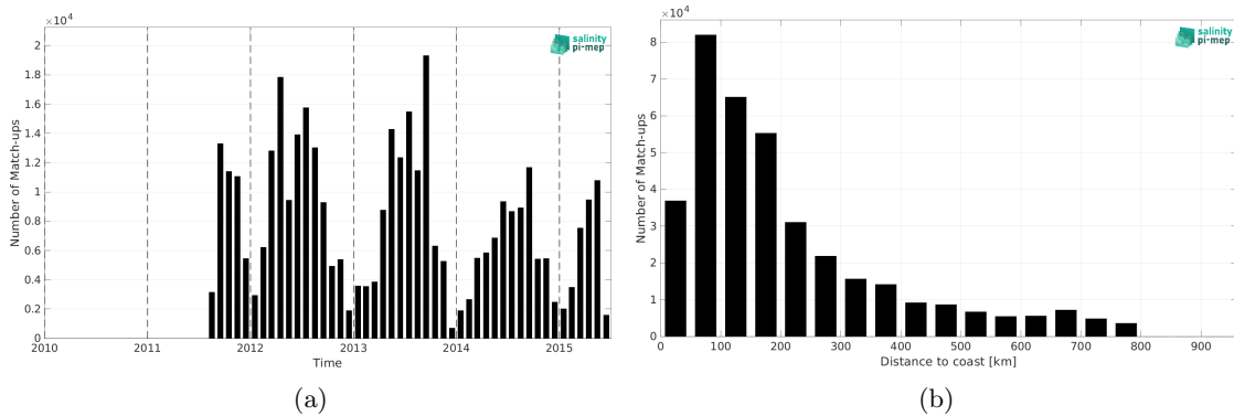
Figure 2: Number of match-ups between TSG (SAMOS) and Aquarius SSS L4 OI v5 - Weekly (IPRC) SSS as a function of time (a) and as function of the distance to coast (b) over the SMOS coastal zone (<800km) 60N-60S Pi-MEP region and for the full satellite product period.
