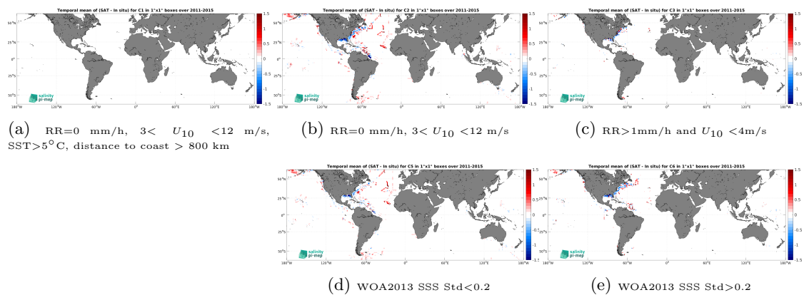
Figure 14: Temporal mean gridded over spatial boxes of size 1^\circ \times 1^\circ of \Delta SSS (Aquarius SSS L4 OI v5 - Weekly (IPRC) - TSG (SAMOS)) for 5 different subdatasets corresponding to:RR=0 mm/h, 3 < U_{10} < 12 m/s, SST >5^\circ\text{C} , distance to coast > 800 km (a), RR=0 mm/h, 3 < U_{10} < 12 m/s (b), RR >1 mm/h and U_{10} < 4 m/s (c), WOA2013 SSS Std <0.2 (d), WOA2013 SSS Std >0.2 (e).
