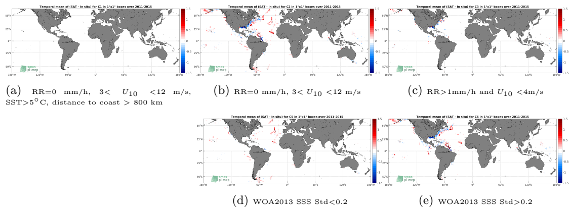
Figure 12: Temporal mean gridded over spatial boxes of size 1^\circ \times 1^\circ of \Delta\text{SSS} (Aquarius SSS L4 OI v5 - Weekly (IPRC) - TSG (SAMOS)) for 5 different subdatasets corresponding to:RR=0 mm/h, 3 < U_{10} < 12 m/s, SST >5^\circ\text{C} , distance to coast > 800 km (a), RR=0 mm/h, 3 < U_{10} < 12 m/s (b), RR >1 mm/h and U_{10} < 4 m/s (c), WOA2013 SSS Std <0.2 (d), WOA2013 SSS Std >0.2 (e).
