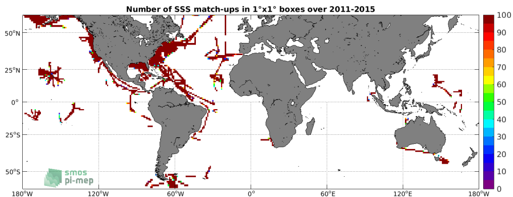
Figure 4: Number of SSS match-ups between TSG (SAMOS) SSS and the Aquarius SSS L4 OI v5 - Weekly (IPRC) SSS product for the SMOS coastal zone (<800km) 60N-60S Pi-MEP region over 1°x1° boxes and for the full satellite product period.
