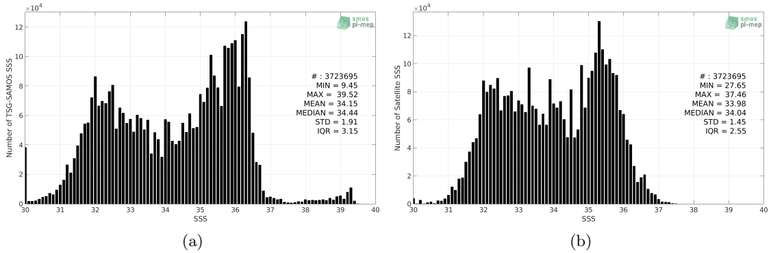
Figure 2: Histograms of SSS from TSG-SAMOS (a) and Aquarius-L4-IPRC-V5-WEEKLY (b) considering all match-up pairs per bins of 0.1 over the SMOS coastal zone ( \geq 800\text{km} ) 60N-60S Pi-MEP region and for the full satellite product period.
