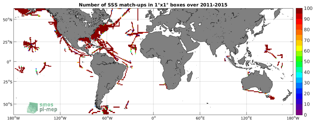
Figure 4: Number of SSS match-ups between TSG-SAMOS SSS and the Aquarius-L4-IPRC-V5-WEEKLY SSS product for the SMOS coastal zone ( \approx 800\text{km} ) 60N-60S Pi-MEP region over 1^\circ \times 1^\circ boxes and for the full satellite product period.
