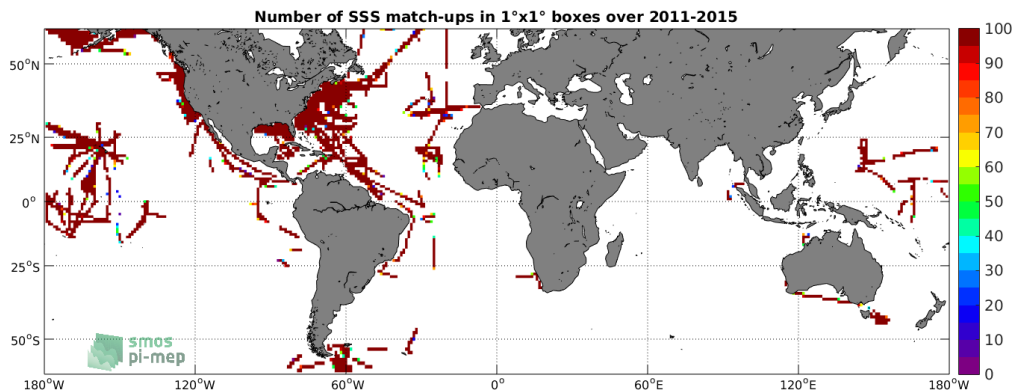
Figure 4: Number of SSS match-ups between TSG-SAMOS SSS and the Aquarius-L4-IPRC-V5-WEEKLY SSS product for the SMOS coastal zone ( \pm 800\text{km} ) 60N-60S Pi-MEP region over 1^\circ \times 1^\circ boxes and for the full satellite product period.
