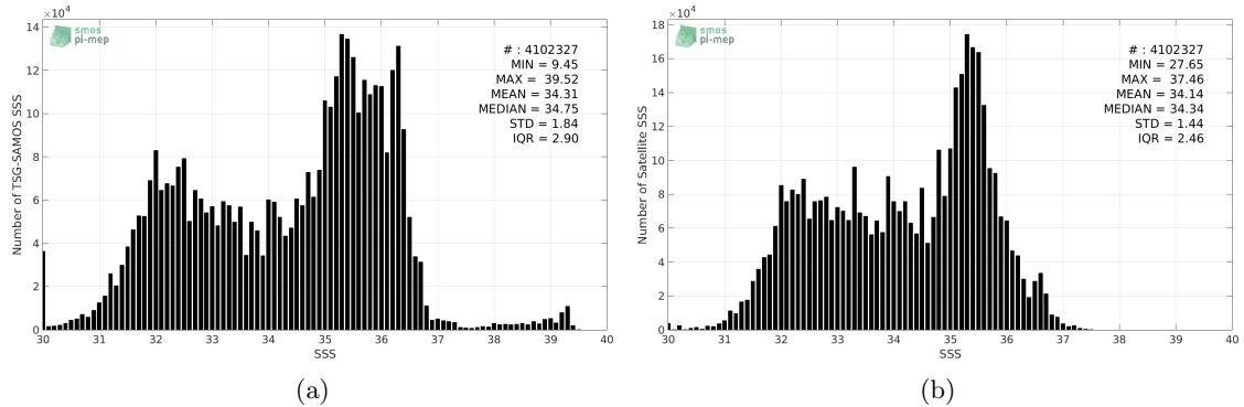
Figure 2: Histograms of SSS from TSG-SAMOS (a) and Aquarius-L4-IPRC-V5-WEEKLY (b) considering all match-up pairs per bins of 0.1 over the SMOS coastal zone ( \approx 800 km) 60N-60S Pi-MEP region and for the full satellite product period.
