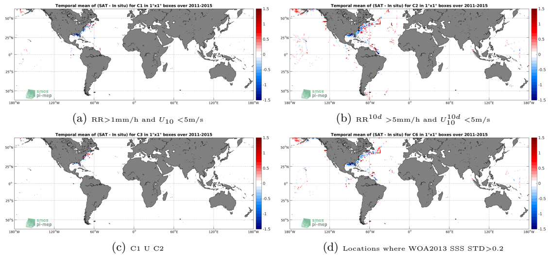
Figure 12: Temporal mean gridded over spatial boxes of size 1^\circ \times 1^\circ of \Delta SSS (Aquarius-L4-IPRC-V5-WEEKLY - TSG-SAMOS) for 4 different subdatasets corresponding to: RR > 1\text{mm/h} and U_{10} < 5\text{m/s} (a), RR^{10d} > 5\text{mm/h} and U_{10}^{10d} < 5\text{m/s} (b), C1 U C2 (c), Locations where WOA2013 SSS STD > 0.2 (d).
