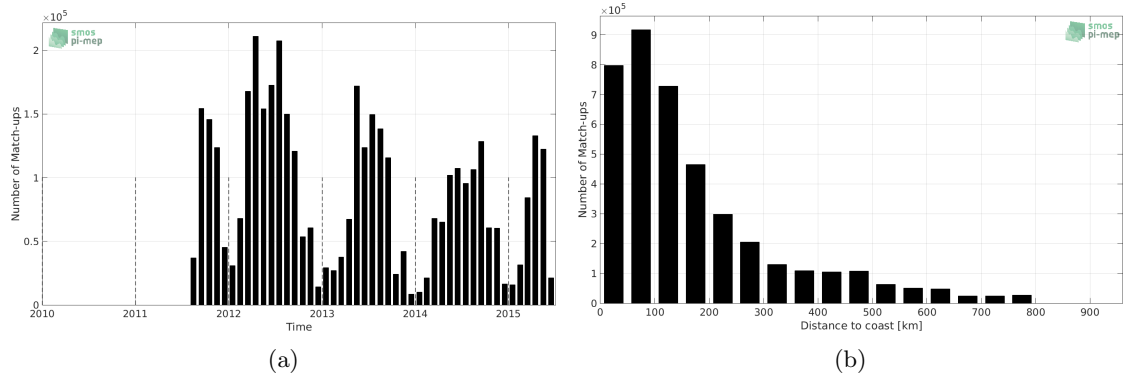
Figure 1: Number of match-ups between TSG-SAMOS and Aquarius-L4-IPRC-V5-WEEKLY SSS as a function of time (a) and as function of the distance to coast (b) over the SMOS coastal zone ( \approx 800 km) 60N-60S Pi-MEP region and for the full satellite product period.
