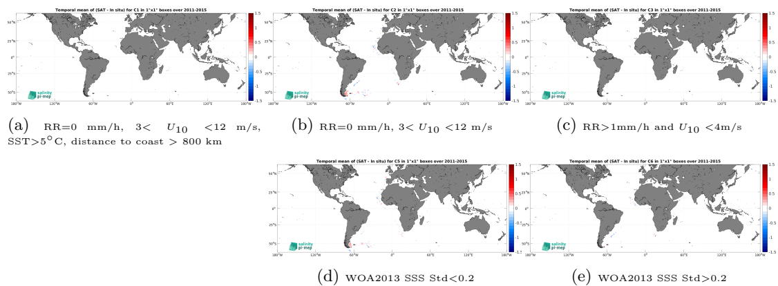
Figure 14: Temporal mean gridded over spatial boxes of size 1^\circ \times 1^\circ of \Delta SSS (Aquarius SSS L4 OI v5 - Weekly (IPRC) - TSG (Polarstern)) for 5 different subdatasets corresponding to:RR=0 mm/h, 3 < U_{10} < 12 m/s, SST >5^\circ\text{C} , distance to coast > 800 km (a), RR=0 mm/h, 3 < U_{10} < 12 m/s (b), RR >1 mm/h and U_{10} < 4 m/s (c), WOA2013 SSS Std <0.2 (d), WOA2013 SSS Std >0.2 (e).
