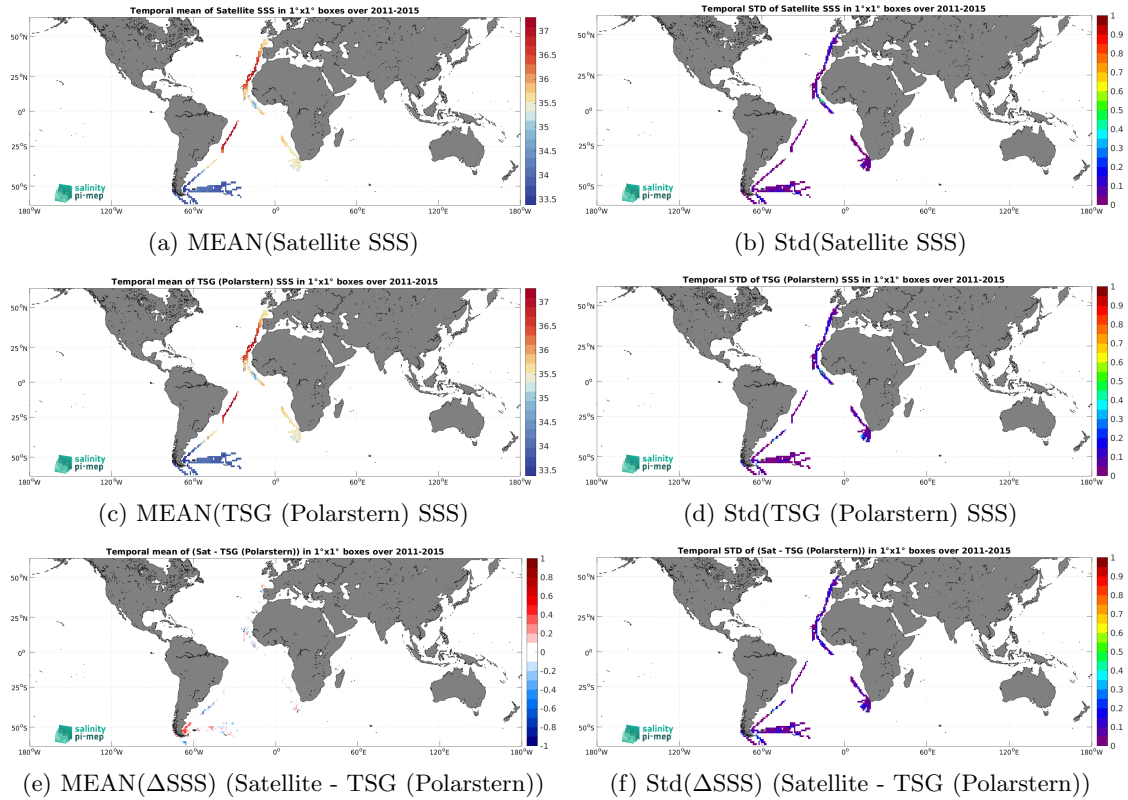
Figure 7: Temporal mean (left) and Std (right) of SSS from Aquarius SSS L4 OI v5 - Weekly (IPRC) (top), TSG (Polarstern) (middle), and of \Delta SSS (Satellite - TSG (Polarstern)). Only match-up pairs are used to generate these maps.
