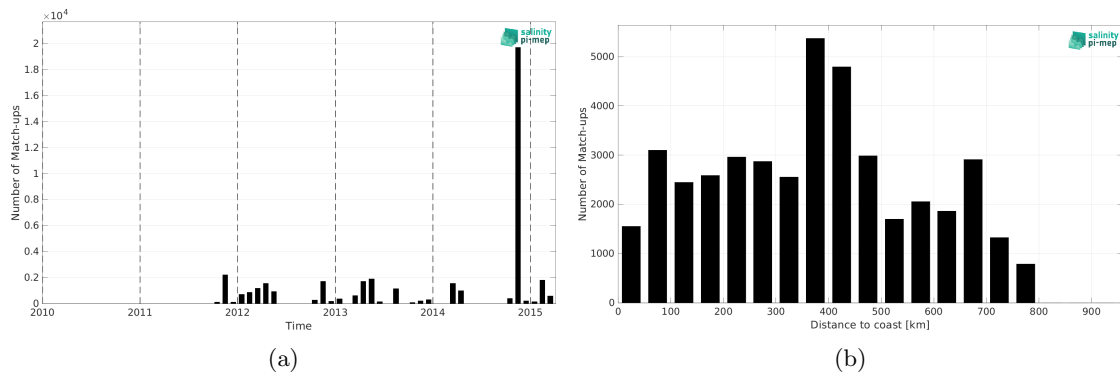
Figure 2: Number of match-ups between TSG (Polarstern) and Aquarius SSS L4 OI v5 - Weekly (IPRC) SSS as a function of time (a) and as function of the distance to coast (b) over the SMOS coastal zone (<800km) 60N-60S Pi-MEP region and for the full satellite product period.
