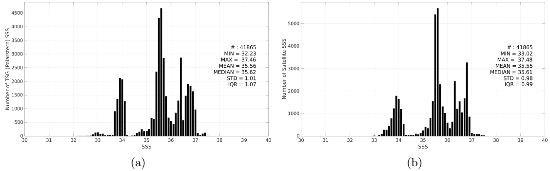
Figure 3: Histograms of SSS from TSG (Polarstern) (a) and Aquarius SSS L4 OI v5 - Weekly (IPRC) (b) considering all match-up pairs per bins of 0.1 over the SMOS coastal zone (<800km) 60N-60S Pi-MEP region and for the full satellite product period.
