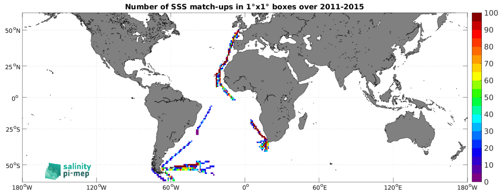
Figure 5: Number of SSS match-ups between TSG (Polarstern) SSS and the Aquarius SSS L4 OI v5 - Weekly (IPRC) SSS product for the SMOS coastal zone (<800km) 60N-60S Pi-MEP region over 1^\circ \times 1^\circ boxes and for the full satellite product period.
