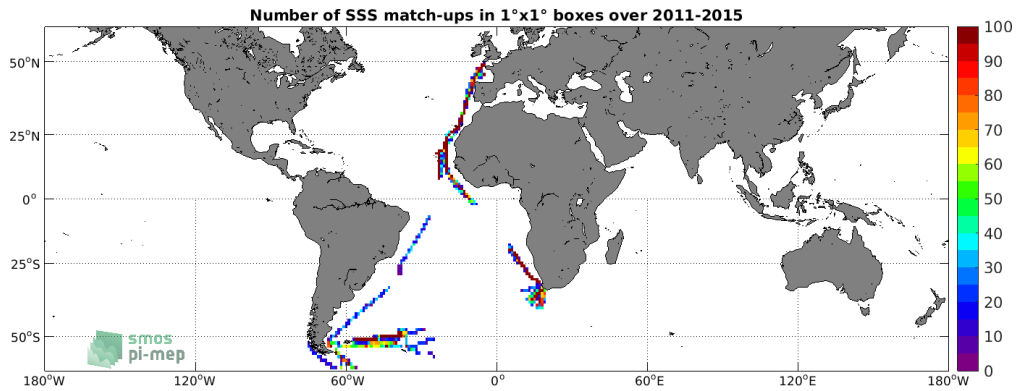
Figure 4: Number of SSS match-ups between TSG (Polarstern) SSS and the Aquarius SSS L4 OI v5 - Weekly (IPRC) SSS product for the SMOS coastal zone (<800km) 60N-60S Pi-MEP region over 1°x1° boxes and for the full satellite product period.
