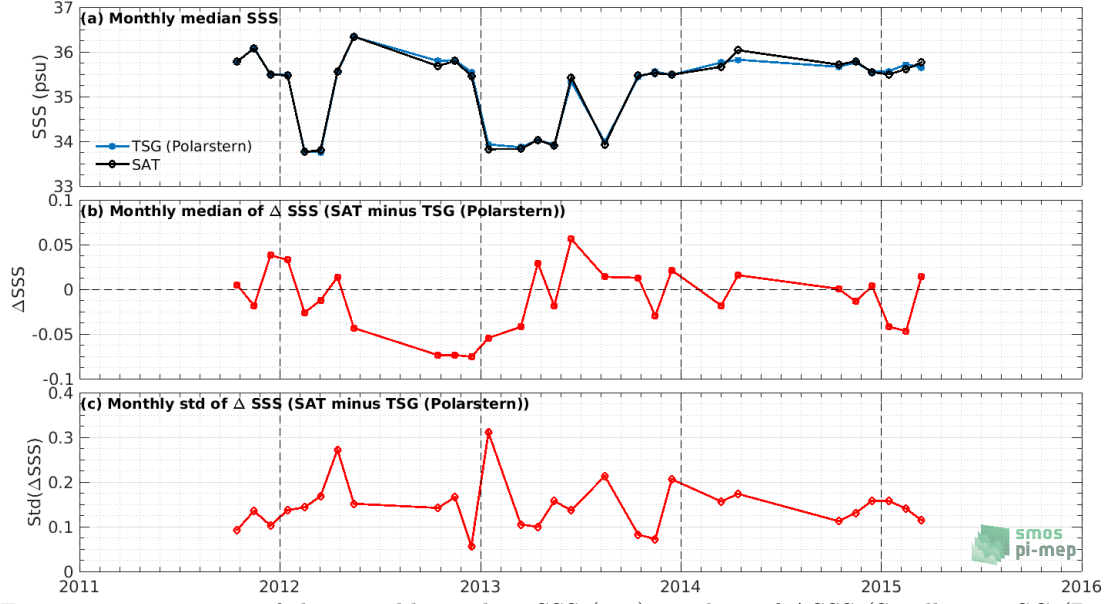
Figure 7: Time series of the monthly median SSS (top), median of \Delta\text{SSS} (Satellite - TSG (Polarstern)) and Std of \Delta\text{SSS} (Satellite - TSG (Polarstern)) over the SMOS coastal zone ( <800\text{km} ) 60N-60S Pi-MEP region considering all match-ups collected by the Pi-MEP.
