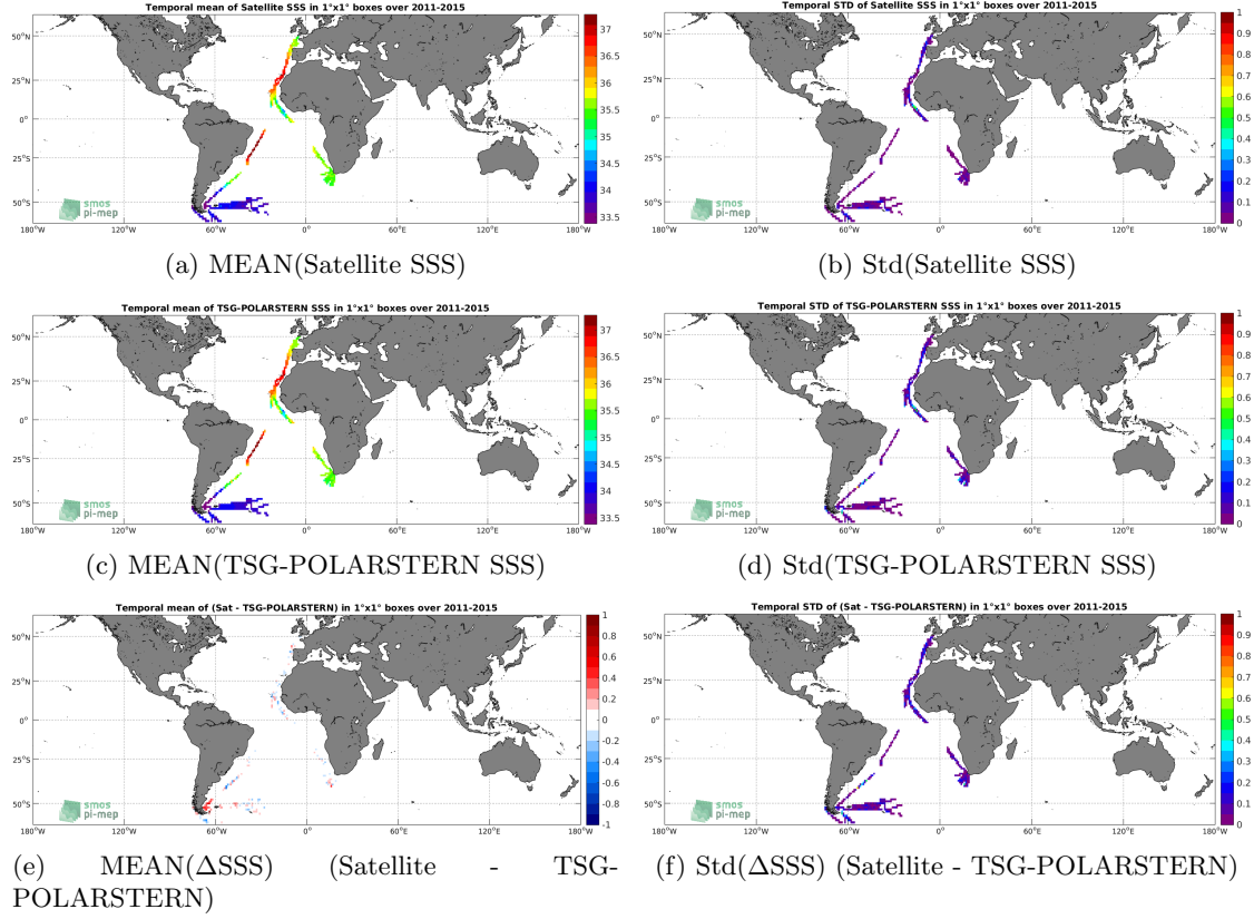
Figure 6: Temporal mean (left) and Std (right) of SSS from Aquarius-L4-IPRC-V5-WEEKLY (top), TSG-POLARSTERN (middle), and of \Delta SSS (Satellite - TSG-POLARSTERN). Only match-up pairs are used to generate these maps.
