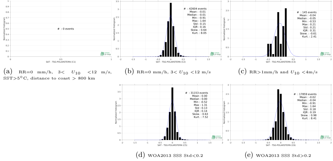
Figure 13: Normalized histogram of \Delta SSS (Aquarius-L4-IPRC-V5-WEEKLY - TSG-POLARSTERN) for 5 different subdatasets corresponding to: RR=0 mm/h, 3 < U_{10} < 12 m/s, SST>5°C, distance to coast > 800 km (a), RR=0 mm/h, 3 < U_{10} < 12 m/s (b), RR>1mm/h and U_{10} < 4 m/s (c), WOA2013 SSS Std<0.2 (d), WOA2013 SSS Std>0.2 (e).
