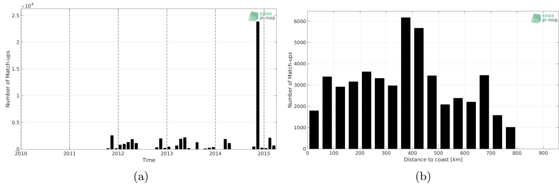
Figure 1: Number of match-ups between TSG-POLARSTERN and Aquarius-L4-IPRC-V5-WEEKLY SSS as a function of time (a) and as function of the distance to coast (b) over the SMOS coastal zone (<800km) 60N-60S Pi-MEP region and for the full satellite product period.
