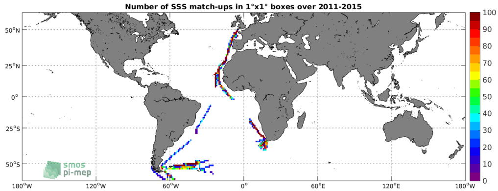
Figure 4: Number of SSS match-ups between TSG-POLARSTERN SSS and the Aquarius-L4-IPRC-V5-WEEKLY SSS product for the SMOS coastal zone (<800km) 60N-60S Pi-MEP region over 1°x1° boxes and for the full satellite product period.
