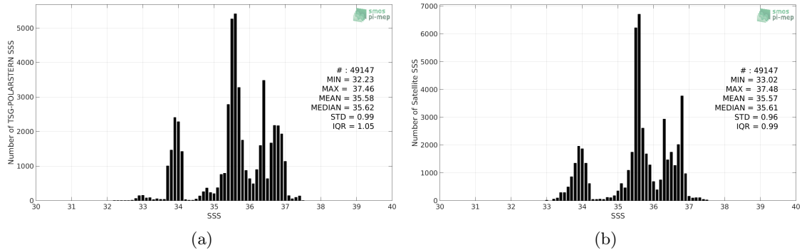
Figure 2: Histograms of SSS from TSG-POLARSTERN (a) and Aquarius-L4-IPRC-V5-WEEKLY (b) considering all match-up pairs per bins of 0.1 over the SMOS coastal zone (<800km) 60N-60S Pi-MEP region and for the full satellite product period.
