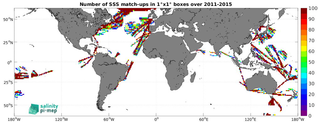
Figure 5: Number of SSS match-ups between TSG (LEGOS-DM) SSS and the Aquarius SSS L4 OI v5 - Weekly (IPRC) SSS product for the SMOS coastal zone (<800km) 60N-60S Pi-MEP region over 1^\circ \times 1^\circ boxes and for the full satellite product period.
