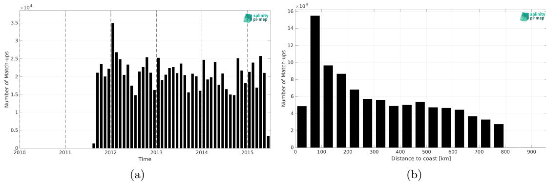
Figure 2: Number of match-ups between TSG (LEGOS-DM) and Aquarius SSS L4 OI v5 - Weekly (IPRC) SSS as a function of time (a) and as function of the distance to coast (b) over the SMOS coastal zone (<800km) 60N-60S Pi-MEP region and for the full satellite product period.
