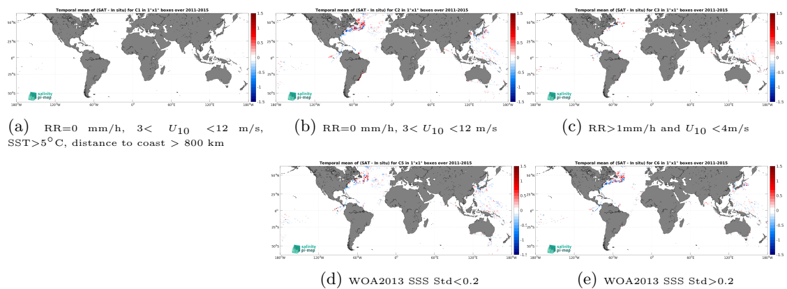
Figure 14: Temporal mean gridded over spatial boxes of size 1^\circ \times 1^\circ of \Delta SSS (Aquarius SSS L4 OI v5 - Weekly (IPRC) - TSG (LEGOS-DM)) for 5 different subdatasets corresponding to:RR=0 mm/h, 3 < U_{10} < 12 m/s, SST >5^\circ\text{C} , distance to coast > 800 km (a), RR=0 mm/h, 3 < U_{10} < 12 m/s (b), RR >1 mm/h and U_{10} < 4 m/s (c), WOA2013 SSS Std <0.2 (d), WOA2013 SSS Std >0.2 (e).
