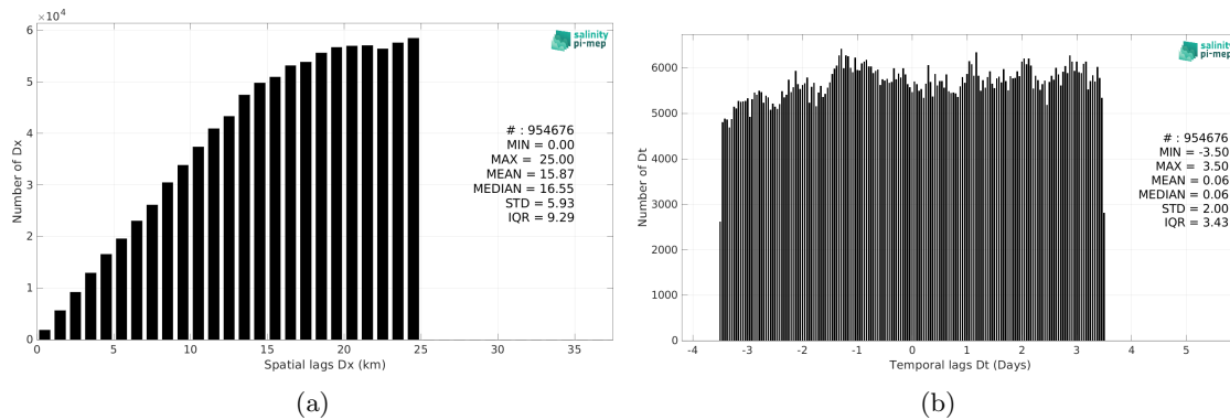
Figure 6: Histograms of the spatial (a) and temporal (b) lags between the location/time of the TSG (LEGOS-DM) measurement and the date of the corresponding Aquarius SSS L4 OI v5 - Weekly (IPRC) SSS pixel.
