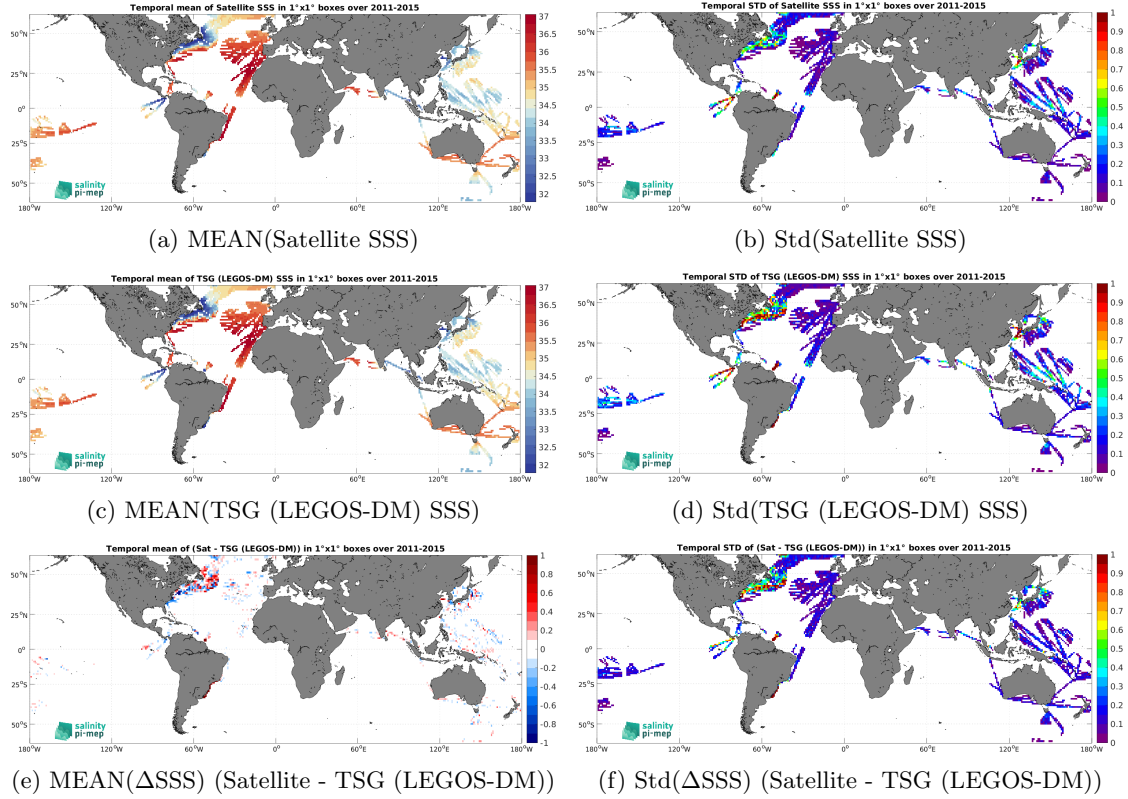
Figure 7: Temporal mean (left) and Std (right) of SSS from Aquarius SSS L4 OI v5 - Weekly (IPRC) (top), TSG (LEGOS-DM) (middle), and of \Delta SSS (Satellite - TSG (LEGOS-DM)). Only match-up pairs are used to generate these maps.
