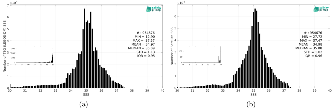
Figure 3: Histograms of SSS from TSG (LEGOS-DM) (a) and Aquarius SSS L4 OI v5 - Weekly (IPRC) (b) considering all match-up pairs per bins of 0.1 over the SMOS coastal zone (<800km) 60N-60S Pi-MEP region and for the full satellite product period.
