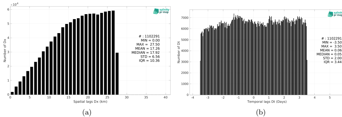
Figure 5: Histograms of the spatial (a) and temporal (b) lags between the location/time of the TSG (LEGOS-DM) measurement and the date of the corresponding Aquarius SSS L4 OI v5 - Weekly (IPRC) SSS pixel.
