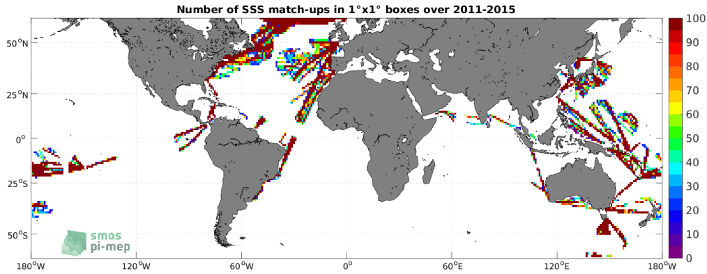
Figure 4: Number of SSS match-ups between TSG (LEGOS-DM) SSS and the Aquarius SSS L4 OI v5 - Weekly (IPRC) SSS product for the SMOS coastal zone (<800km) 60N-60S Pi-MEP region over 1^\circ \times 1^\circ boxes and for the full satellite product period.
