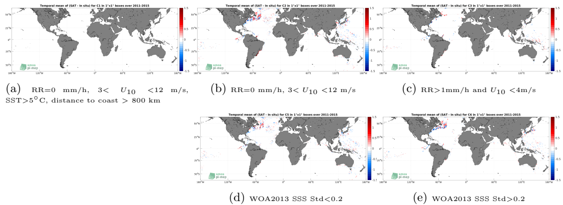
Figure 12: Temporal mean gridded over spatial boxes of size 1^\circ \times 1^\circ of \Delta SSS (Aquarius SSS L4 OI v5 - Weekly (IPRC) - TSG (LEGOS-DM)) for 5 different subdatasets corresponding to:RR=0 mm/h, 3 < U_{10} < 12 m/s, SST >5^\circ\text{C} , distance to coast > 800 km (a), RR=0 mm/h, 3 < U_{10} < 12 m/s (b), RR >1 mm/h and U_{10} < 4 m/s (c), WOA2013 SSS Std <0.2 (d), WOA2013 SSS Std >0.2 (e).
