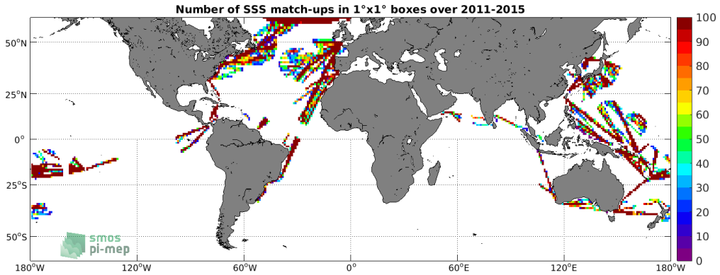
Figure 4: Number of SSS match-ups between TSG (LEGOS-DM) SSS and the Aquarius SSS L4 OI v5 - Weekly (IPRC) SSS product for the SMOS coastal zone (<800km) 60N-60S Pi-MEP region over 1°x1° boxes and for the full satellite product period.
