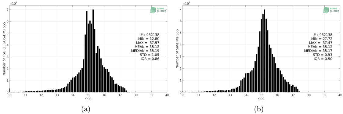
Figure 2: Histograms of SSS from TSG (LEGOS-DM) (a) and Aquarius SSS L4 OI v5 - Weekly (IPRC) (b) considering all match-up pairs per bins of 0.1 over the SMOS coastal zone (<800km) 60N-60S Pi-MEP region and for the full satellite product period.
