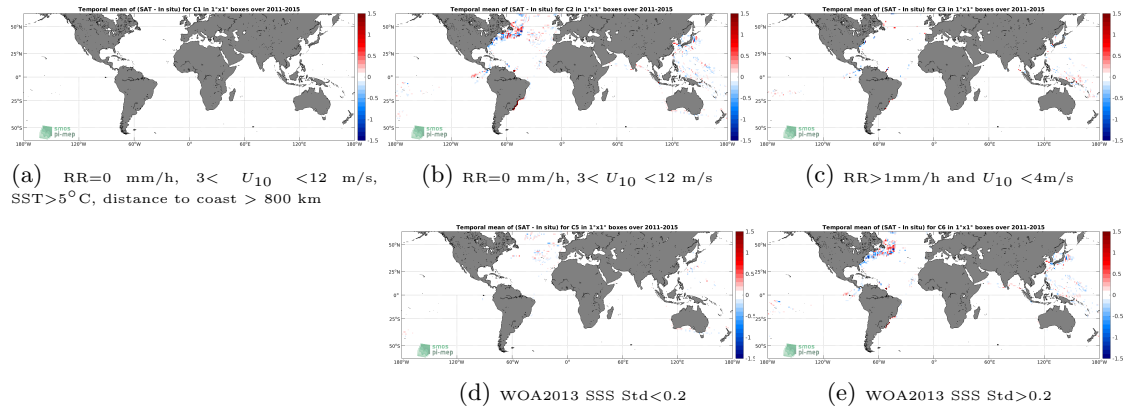
Figure 12: Temporal mean gridded over spatial boxes of size 1^\circ \times 1^\circ of \Delta SSS (Aquarius SSS L4 OI v5 - Weekly (IPRC) - TSG (LEGOS-DM)) for 5 different subdatasets corresponding to: RR=0 mm/h, 3 < U_{10} < 12 m/s, SST > 5^\circ C , distance to coast > 800 km (a), RR=0 mm/h, 3 < U_{10} < 12 m/s (b), RR > 1 mm/h and U_{10} < 4 m/s (c), WOA2013 SSS Std < 0.2 (d), WOA2013 SSS Std > 0.2 (e).
