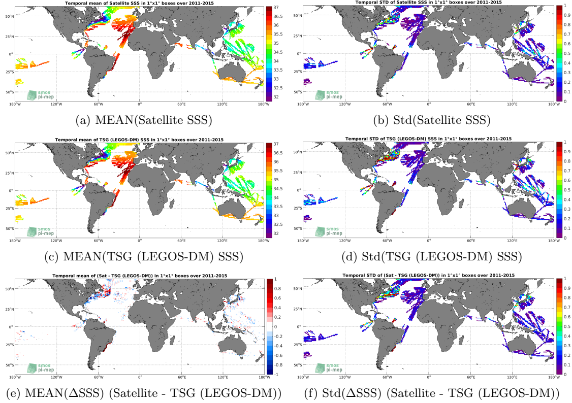
Figure 6: Temporal mean (left) and Std (right) of SSS from Aquarius SSS L4 OI v5 - Weekly (IPRC) (top), TSG (LEGOS-DM) (middle), and of \Delta SSS (Satellite - TSG (LEGOS-DM)). Only match-up pairs are used to generate these maps.
