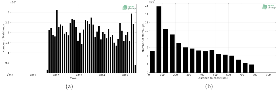
Figure 1: Number of match-ups between TSG (LEGOS-DM) and Aquarius SSS L4 OI v5 - Weekly (IPRC) SSS as a function of time (a) and as function of the distance to coast (b) over the SMOS coastal zone (<800km) 60N-60S Pi-MEP region and for the full satellite product period.
