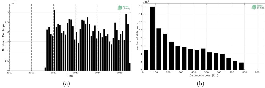
Figure 1: Number of match-ups between TSG-LEGOS-DM and Aquarius-L4-IPRC-V5-WEEKLY SSS as a function of time (a) and as function of the distance to coast (b) over the SMOS coastal zone (<800km) 60N-60S Pi-MEP region and for the full satellite product period.
