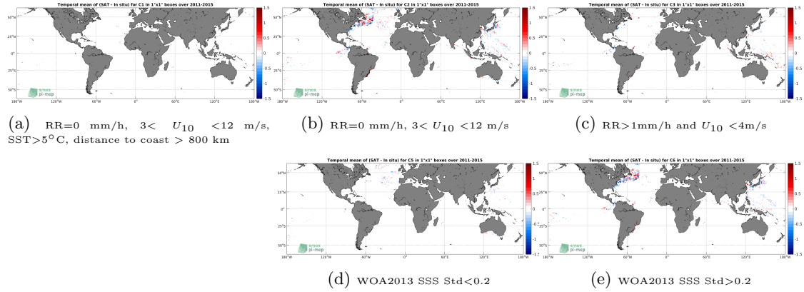
Figure 12: Temporal mean gridded over spatial boxes of size 1^\circ \times 1^\circ of \Delta SSS (Aquarius-L4-IPRC-V5-WEEKLY - TSG-LEGOS-DM) for 5 different subdatasets corresponding to: RR=0 mm/h, 3 < U_{10} < 12 m/s, SST > 5^\circ C , distance to coast > 800 km (a), RR=0 mm/h, 3 < U_{10} < 12 m/s (b), RR > 1 mm/h and U_{10} < 4 m/s (c), WOA2013 SSS Std < 0.2 (d), WOA2013 SSS Std > 0.2 (e).
