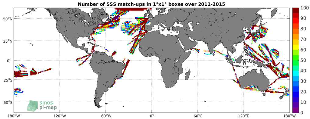
Figure 4: Number of SSS match-ups between TSG-LEGOS-DM SSS and the Aquarius-L4-IPRC-V5-WEEKLY SSS product for the SMOS coastal zone (<800km) 60N-60S Pi-MEP region over 1°x1° boxes and for the full satellite product period.
