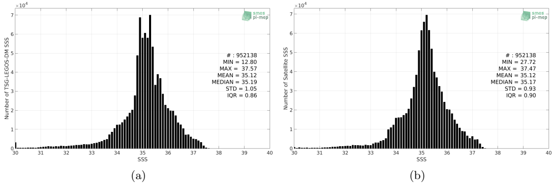
Figure 2: Histograms of SSS from TSG-LEGOS-DM (a) and Aquarius-L4-IPRC-V5-WEEKLY (b) considering all match-up pairs per bins of 0.1 over the SMOS coastal zone (<800km) 60N-60S Pi-MEP region and for the full satellite product period.
