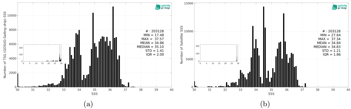
Figure 3: Histograms of SSS from TSG (GOSUD-Sailing-ship) (a) and Aquarius SSS L4 OI v5 - Weekly (IPRC) (b) considering all match-up pairs per bins of 0.1 over the SMOS coastal zone (<800km) 60N-60S Pi-MEP region and for the full satellite product period.
