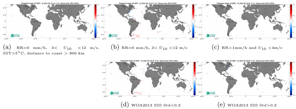
Figure 14: Temporal mean gridded over spatial boxes of size 1^\circ \times 1^\circ of \Delta SSS (Aquarius SSS L4 OI v5 - Weekly (IPRC) - TSG (GOSUD-Sailing-ship)) for 5 different subdatasets corresponding to:RR=0 mm/h, 3 < U_{10} < 12 m/s, SST >5^\circ\text{C} , distance to coast > 800 km (a), RR=0 mm/h, 3 < U_{10} < 12 m/s (b), RR >1 mm/h and U_{10} < 4 m/s (c), WOA2013 SSS Std <0.2 (d), WOA2013 SSS Std >0.2 (e).
