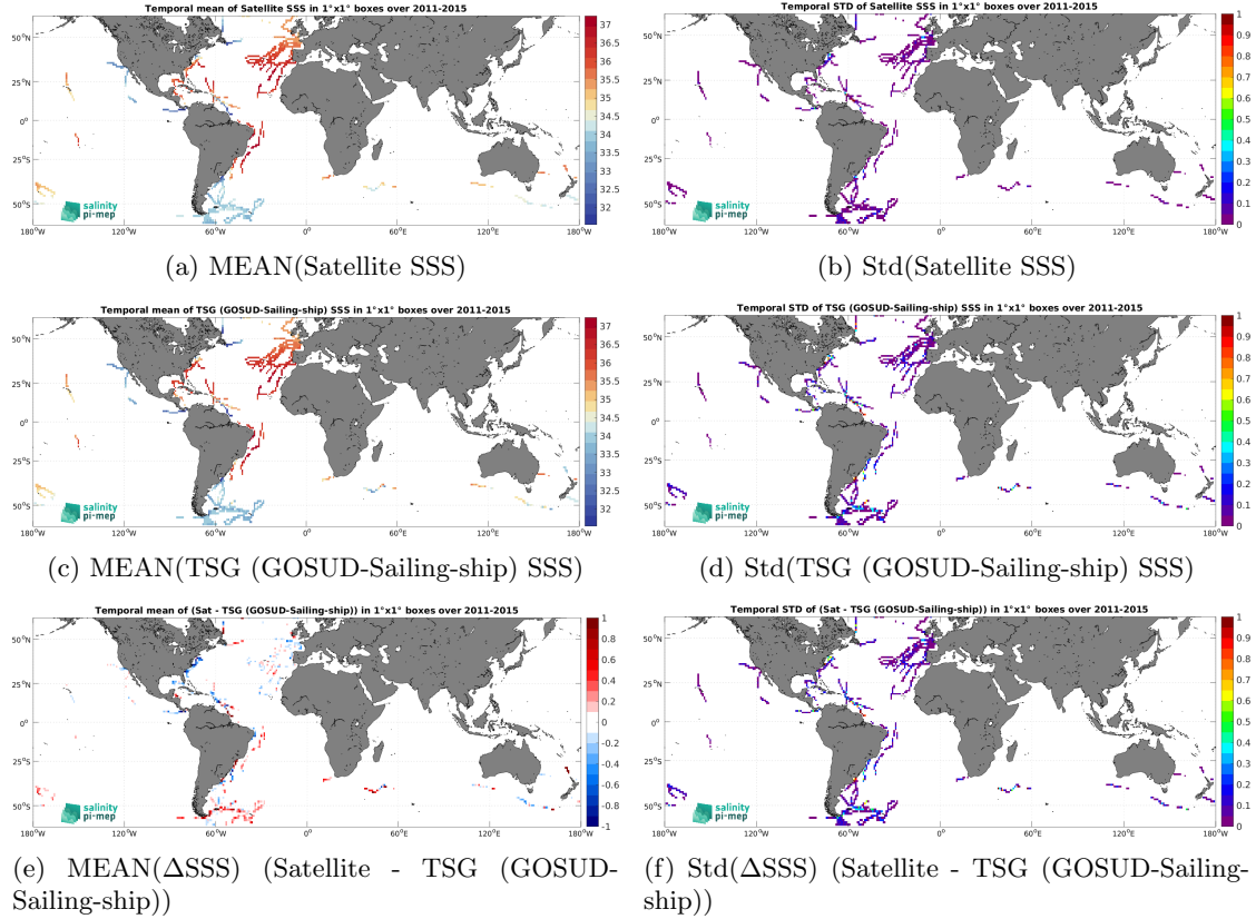
Figure 7: Temporal mean (left) and Std (right) of SSS from Aquarius SSS L4 OI v5 - Weekly (IPRC) (top), TSG (GOSUD-Sailing-ship) (middle), and of \Delta SSS (Satellite - TSG (GOSUD-Sailing-ship)). Only match-up pairs are used to generate these maps.
