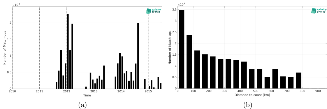
Figure 2: Number of match-ups between TSG (GOSUD-Sailing-ship) and Aquarius SSS L4 OI v5 - Weekly (IPRC) SSS as a function of time (a) and as function of the distance to coast (b) over the SMOS coastal zone (<800km) 60N-60S Pi-MEP region and for the full satellite product period.
