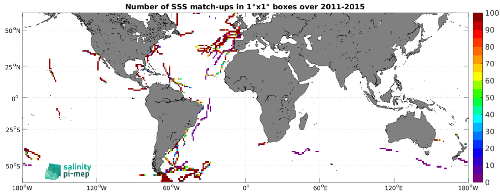
Figure 5: Number of SSS match-ups between TSG (GOSUD-Sailing-ship) SSS and the Aquarius SSS L4 OI v5 - Weekly (IPRC) SSS product for the SMOS coastal zone (<800km) 60N-60S Pi-MEP region over 1^{\circ} \times 1^{\circ} boxes and for the full satellite product period.
